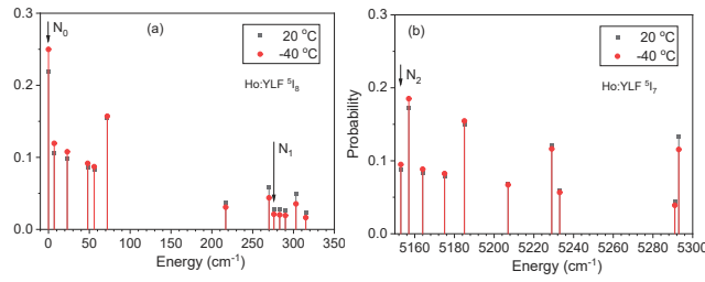
Fig. 1. Boltzmann fractions of the (a) ^5I_8 and (b) ^5I_7 levels of Ho:YLF at two temperatures, 20 °C and -40 °C. N_0 , N_1 , and N_2 are the ground state, lower, and upper laser levels, respectively, for amplifying signals at 2.05 \mu\text{m} .
