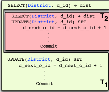
Fig. 3. An RC execution involving two instances ( T_1 and T_2 ) of the new_order transaction depicted in Fig. 1. Both instances read the d\_id District record concurrently, because neither transaction is committed when the reads are executed. The subsequent operations are effectively sequentialized, since T_2 commits before T_1 . Nonetheless, both transactions read the same value for d\_next\_o\_id resulting in them adding Order records with the same ids, which in turn triggers a violation of TPC-C's consistency condition.
