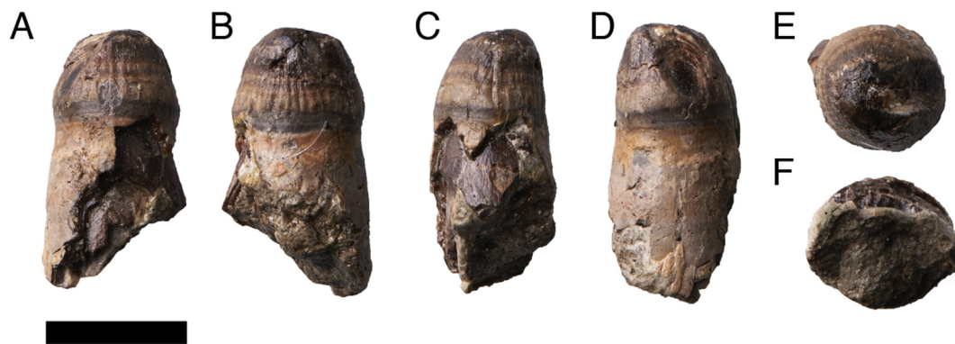
Fig. 9. An isolated molariform tooth of Yanjisuchus longshanensis gen. et sp. nov., holotype (YJDM 00009) in labial (A), lingual (B), anterior (C), posterior (D), apical (E), and basal (F) views. Scale bar = 1 cm.
