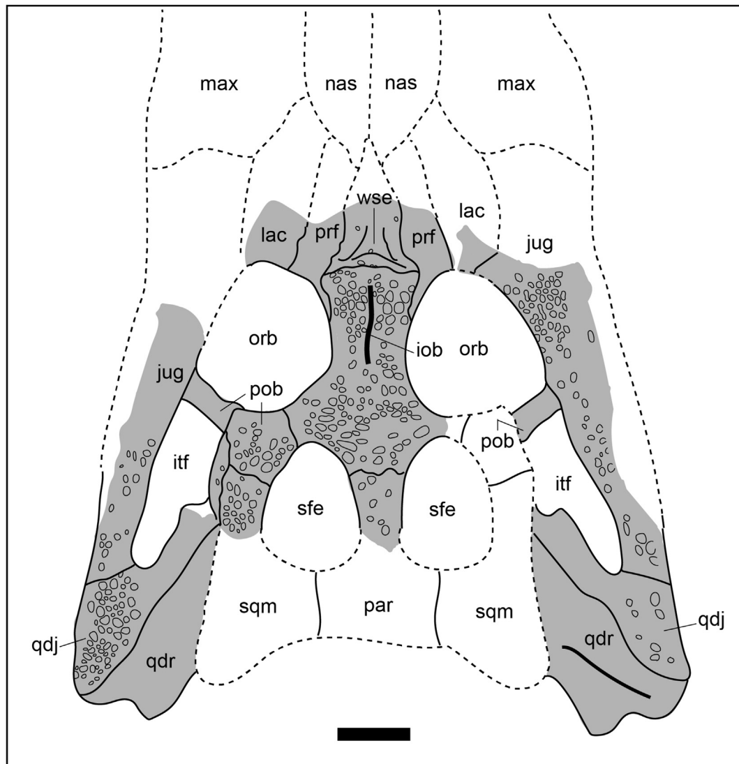
Fig. 7. Reconstruction of the preserved skull elements of Yanjisuchus longshanensis gen. et sp. nov., holotype (YJDM 00009) in dorsal view. Solid lines and areas in gray indicate the preserved parts. Scale bar = 2 cm.
