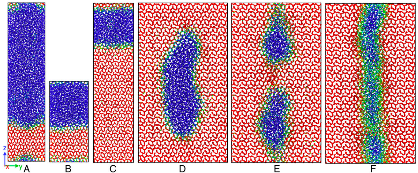
Fig. 4. Modeling volume fraction and interface effects of HDA and ice VI in MD simulations. (A–C) Ice VI and HDA sandwich systems with different initial phase volume fraction of (A) \frac{N_{VI}}{N_{HDA}} = \frac{1}{3} (B) \frac{N_{VI}}{N_{HDA}} = 1 , and (C) \frac{N_{VI}}{N_{HDA}} = 3 . (D–F) Ice VI and HDA-embedded systems with initial \frac{N_{VI}}{N_{HDA}} = 2.23 and with increasing interface volume, from left to right. Ice VI, ice HDA, and the interfacial regions are distinguished by red, blue, and green, respectively.
