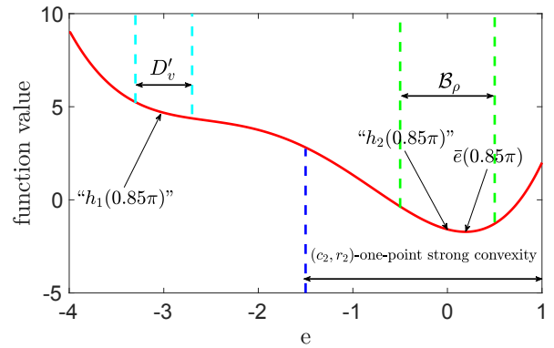
Fig. 6. Illustration of Definition 9: the region of domination.
