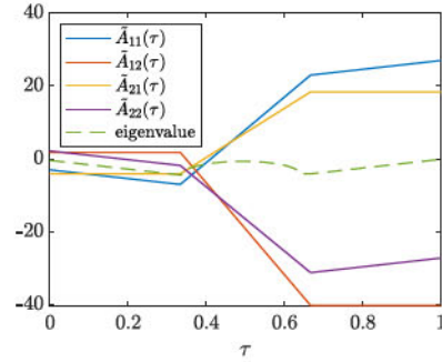
Fig. 7. Stable path between the two matrices \bar{A}(0) and \bar{A}(1) in Example 3. The curve labeled “eigenvalue” shows the maximum real part of the eigenvalues for the corresponding matrices on the path.
