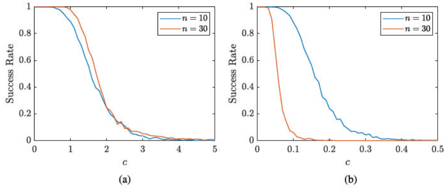
Fig. 3. Success rate of Algorithm 1 on random examples with different values for n and c .
