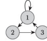
Fig. 1. Graph representation of the pattern (3).
