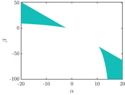
Fig. 4. Feasible region of the ODC problem in Example 2.
