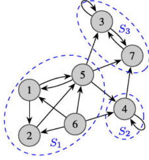
Fig. 2. Complement graph of the pattern studied in Example 1.
