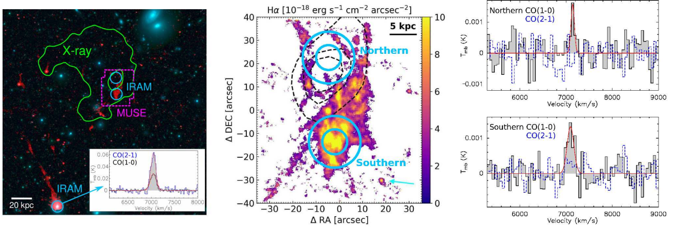
Fig. 1. Multiwavelength observations of the A1367 OC. Left: A1367 OC – the green contour outlines its X-ray morphology (0.5–2 keV XMM observations) overlaid on a Subaru three-color composite image (red, H \alpha ; green, r -band; and blue, g -band). The dashed magenta region shows the MUSE FOV, and the blue circles indicate the IRAM CO(1-0) beams. Image adapted from Ge et al. (2021). The galaxy 2MASX J11443212+2006238 with its 85 kpc long H \alpha ram pressure stripped tail is visible to the south of the OC. The CO spectra from a pointing centered on this galaxy are shown in the inset. Middle: MUSE H \alpha image of the OC (Ge et al. 2021) showing the positions of the CO(1-0) and CO(2-1) beams (blue circles, HPBW of 21.7'' \approx 9.7 kpc and 10.9'' \approx 4.9 kpc, respectively). The black dashed contours show the peak X-ray emission of the OC. Right: CO(1-0) lines detected at the positions over the northern X-ray peak ( top panel ) and the southern H \alpha peak ( bottom panel ). Velocity corresponds to v_{\text{rad}} = cz/(z + 1) . The corresponding CO(2-1) spectra divided by a factor of 3 are shown with dotted blue lines. In the southern region ( bottom panel ), a marginal CO(2-1) line detection is suggested from a positive signal at velocities around the CO(1-0) line central velocity.
