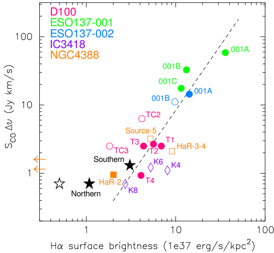
Fig. 2. CO integrated flux vs. H \alpha surface brightness measured in a sample of ram pressure stripped gas tails (Jáchym et al. 2017, their Fig. 9). The location of the two OC regions is shown with filled stars. The open star symbol corresponds to the northern region surface brightness, when the full area of the CO(1-0) beam is used instead of the actual H \alpha -emitting area within the beam (filled star).
