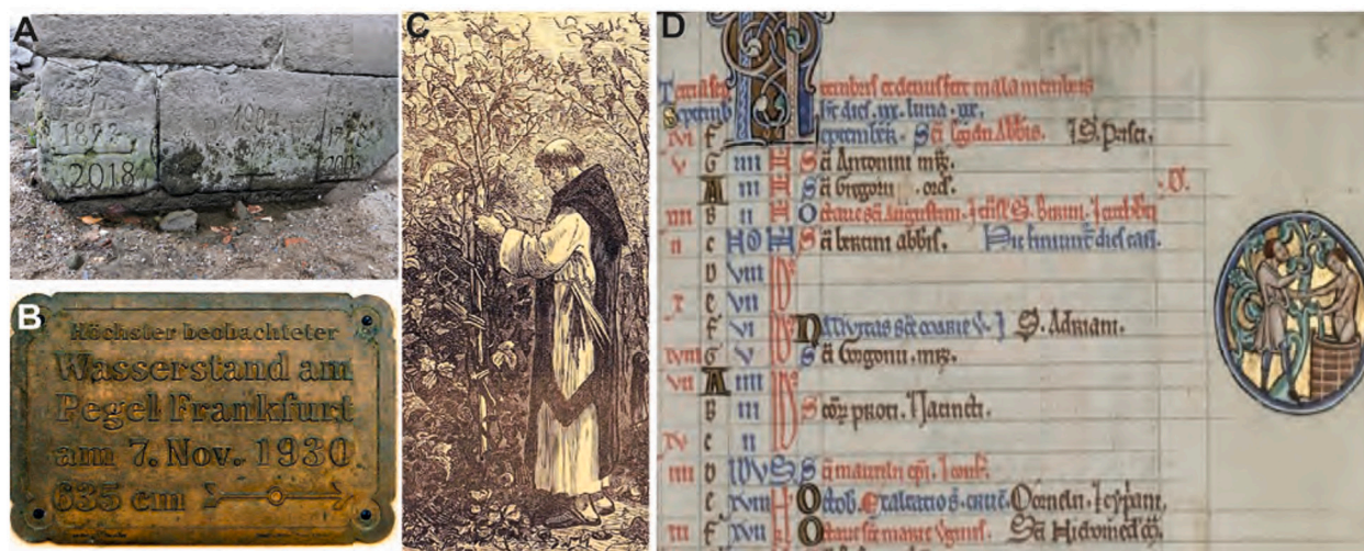
Fig. 2. Historical archives and their relation to seasonality. A: drought marker (‘Hungerstein’) at Elbe river, Dresden, South-East Germany; B: flood marker at the Oder river, Frankfurt, East Germany; C: Illustration of monks harvesting wine in Bourgogne, France at the end of 19th c. D: September calendar showing Grape harvest and wine pressing. Photos A and B mark historical floods or droughts along rivers. The study of compiled historical markers as indirect proxies for seasonality give insights in changes in season’s dynamics and trends. More frequent drought events during certain periods might reflect hot/longer summer seasons, whereas recurrent flood events can reflect severe/longer winter or spring season with higher amount of water/snow melt. Fig. C is an extract B.11.4 (f. v recto.) of ‘Psalterium’, a manuscript from the 13th c., in which M.R. James describes the scene thus: “Cuts grapes from vine with sickle and holds the hand of a nude man in a vat.” From the James Catalogue of Western Manuscripts, digital library of the Trinity College, Cambridge. All photos are under CC licence.
