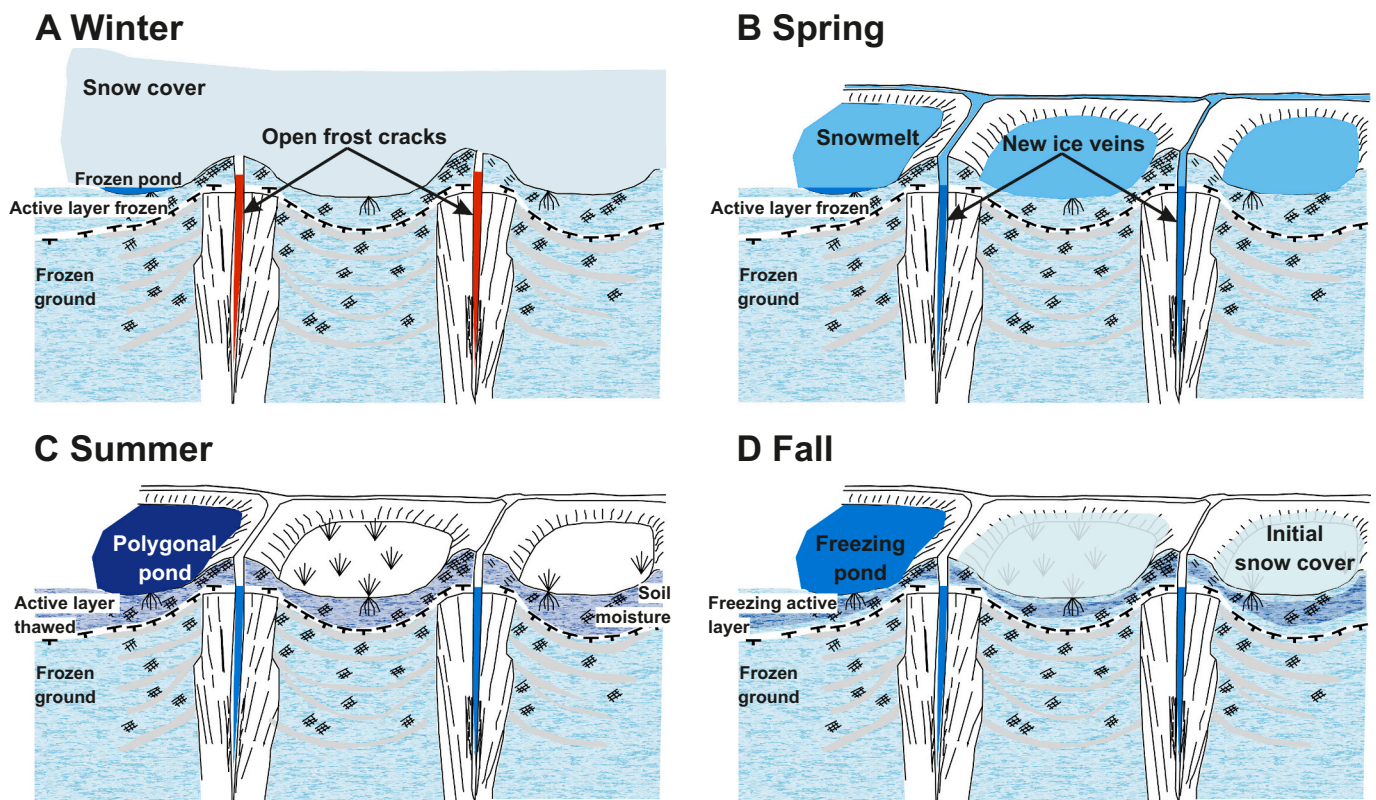
Fig. 14. Schematic overview of relevant seasonal processes leading to the formation of ice wedges and pore ice as climate archives. A: Winter. Accumulation of snow cover subject to sublimation and wind drift, frost cracks open. B: Spring. Snowmelt refreezes in frost cracks and forms new ice veins. C: Summer. Soil moisture in the thawed active layer integrates melt water and precipitation subject to evaporation. D: Fall. Active layer freezes and soil moisture turns into pore ice, initial snow cover.
