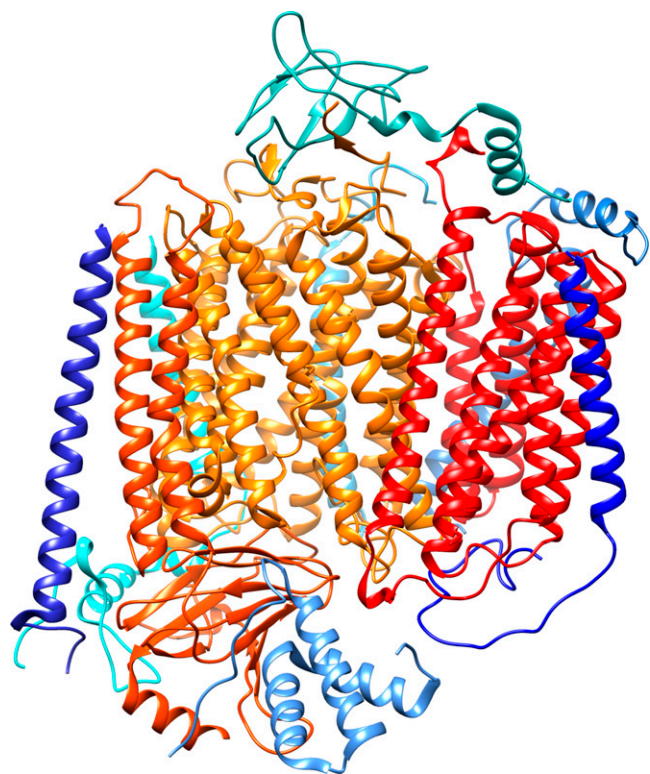
Fig. 1. Structure of cytochrome c oxidase from the angiosperm Vigna radiata (71). Mitochondrial-encoded subunits Cox1, Cox2, and Cox3 are shown in shades of orange to red. Nuclear-encoded subunits are shown in shades of blue. All subunits assemble in an equimolar ratio with each present in a single copy within the complex. The image was generated with Chimera v1.15 (72), using Protein Data Bank accession 7JRO.
