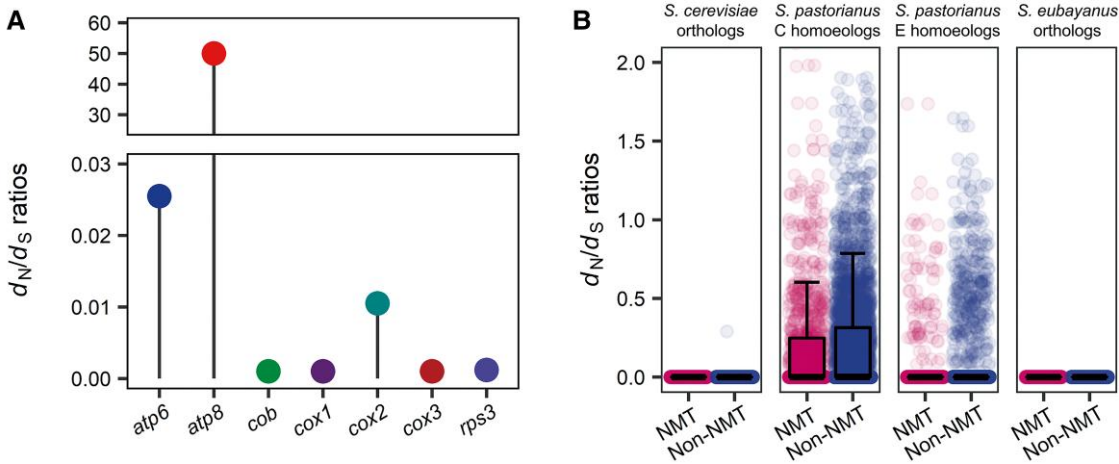
Fig. 1. Nonsynonymous to synonymous substitution ratios ( d_N/d_S ) of mitochondrial and nuclear genes. (A) d_N/d_S ratios (y-axis) of homologous mitochondrial genes (mtDNA genes; x-axis) in S. pastorianus and S. eubayanus are summarized; (B) Each panel summarizes the d_N/d_S ratios of all single-copy NMT and non-NMT genes characterized in diploid orthologs of S. eubayanus and S. cerevisiae and subgenomic homoeologs of allopolyploid S. pastorianus .
