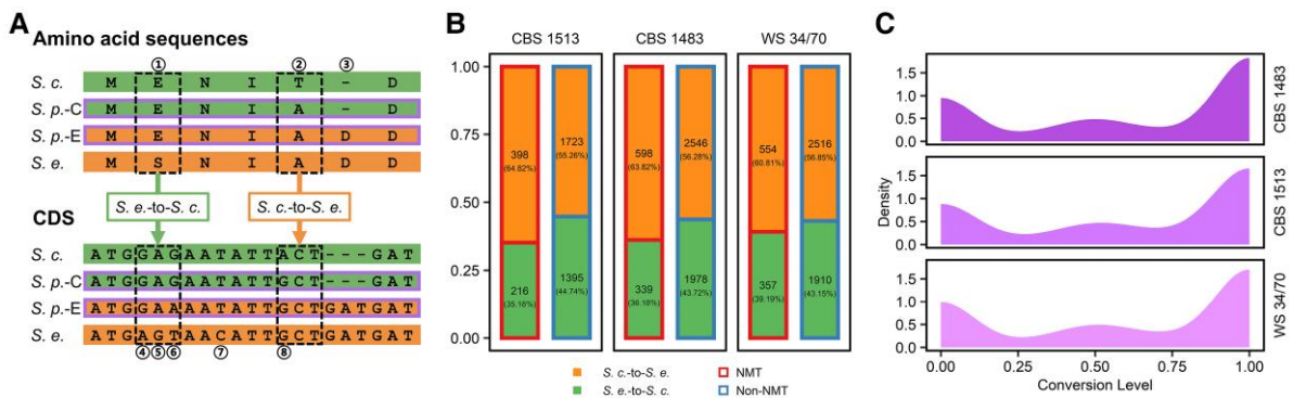
FIG. 2. Genetic cytonuclear coordination in three allopolyploid S. pastorianus strains. (A) Schematic diagram illustrating the S. cerevisiae -to- S. eubayanus ( S. c.-to-S. e. ) and S. eubayanus -to- S. cerevisiae ( S. e.-to-S. c. ) gene conversions (in right and left dotted boxes). Single-copy gene orthologs and homoeologs (C and E subgenomes) are aligned into quartets. Changes of amino acids and nucleotides involved in gene conversion are specified in each box. Labels 1–8 describe the criteria of defining nonsynonymous gene conversions among homoeologs (see Materials and Methods); (B) Number and relative percentage of S. cerevisiae -to- S. eubayanus ( S. c.-to-S. e. ) and S. eubayanus -to- S. cerevisiae ( S. e.-to-S. c. ) gene conversions in NMT and non-NMT homoeologs in three S. pastorianus strains are summarized in each column. (C) Density distribution of gene conversion levels of identified S. cerevisiae -to- S. eubayanus ( S. c.-to-S. e. ) gene conversions in each S. pastorianus strain.
