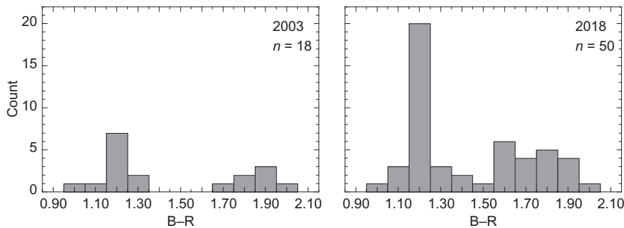
FIG. 14.2 Centaur B–R histograms as they were in 2003 and as they are in 2018 from TRC data. In the larger 2018 sample, the red population became broader and the gap between the gray and red populations became a dip. Note that we are using the more strict definition of Centaurs.
