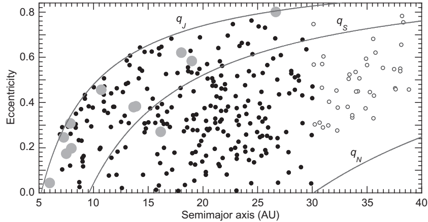
FIG. 14.1 Semimajor axis and eccentricity plot of known Centaurs. Large gray dots indicate known active Centaurs. Black dots indicate Centaurs with both perihelion and semimajor axis between those of Jupiter and Neptune, that is, the more strict definition. White dots indicate objects classified as Centaurs by DES alone. The curves where objects have perihelion equal to the semimajor axis of Jupiter, q_J , of Saturn, q_S , and of Neptune, q_N , are drawn. Several objects are out of scale.
