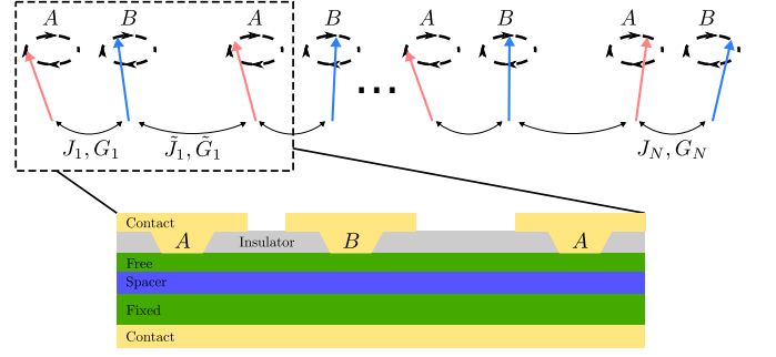
FIG. 1. Schematic illustration of the model considered in this work. The array of STOs is represented as a 1D lattice with a two-sublattice (A and B) unit cell. The STOs are connected via a metallic spacer that mediates an intra-cell ( J_i, G_i ) and inter-cell ( \tilde{J}_i, \tilde{G}_i ) complex nearest-neighbor hopping. The inset shows a possible experimental realization of the STOs array, with the stacking of contact|fixed layer|spacer|free layer|contact. The magnetic layers extend throughout the array, and spin waves excited by one STO can reach and dissipatively couple the neighboring STOs.
