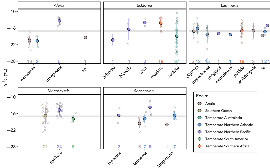
Figure 6. Taxonomic variation in kelp \delta^{13}\text{C} values worldwide. Kelp \delta^{13}\text{C} values (blades only) are organized by the five most widely sampled genera and presented at the species level. All raw values from the literature are shown as translucent points with larger points representing mean \pm SD. For taxa with only one unique observation the data point represents the mean reported in the study. For taxa with only two observations the mean represents the average of those two studies. Points are colored by realm (as defined by Spalding et al. 2007) and the numbers along the x-axis indicate the total number of \delta^{13}\text{C} values obtained from the literature.
