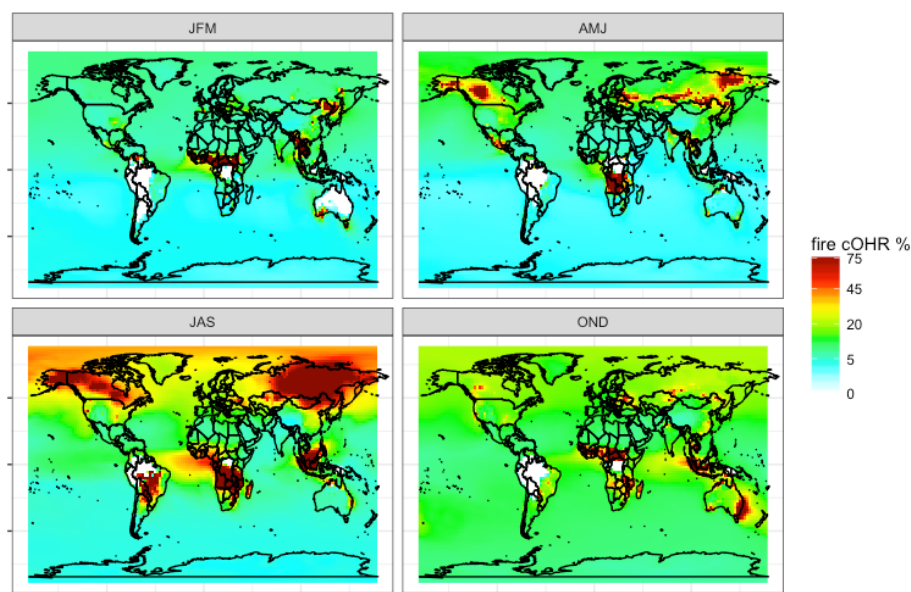
Figure 8. Percent surface cOHR seasonally from fires in 2019 from updated GEOS-Chem simulation (see Sect. 3) using GFED4s DM with Andreae (2019) emission factors. JFM is January, February, March; AMJ is April, May, June; JAS is July, August, September; and OND is October, November, December.
