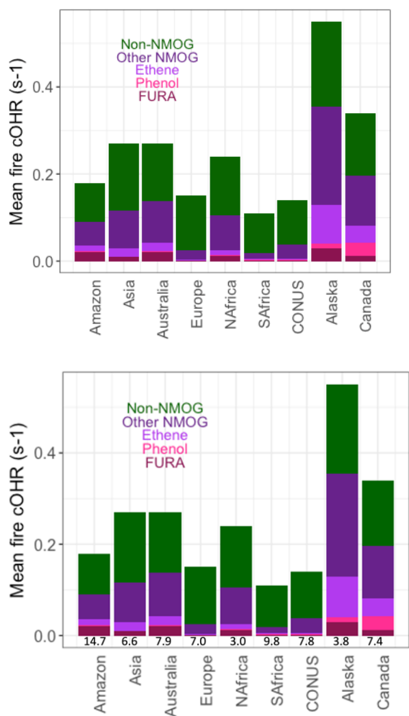
Figure 10: Mean simulated surface fire cOHR in 2019 using GFED4s DM regionally for the Amazon, Asia, Australia, Europe, northern hemispheric Africa (NAfrica), southern hemispheric Africa (SAfrica), the contiguous US (CONUS), Alaska, and Canada. Numbers at the bottom of each bar are the 1997-2016 area-averaged burned area in Mkm 2 from van der Werf et al. (2017). See Fig. S9 for the same analysis with the standard model.
