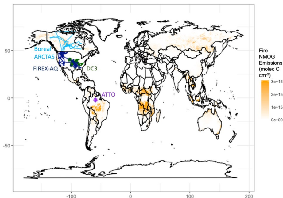
Figure 2. Measurement locations of campaigns used in this analysis overlaid on annual mean NMOG emissions from fires across 1997 – 2019 from GFED4s. Boreal ARCTAS is in light blue, FIREX-AQ in dark blue, DC3 in dark green, and ATTO in purple.
