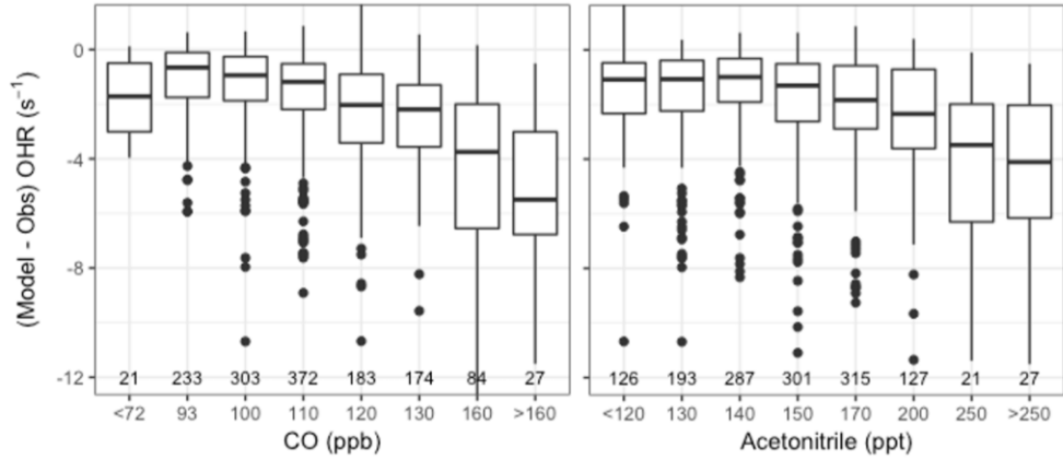
Figure 6. Boxplots of the model minus observed OHR or OHR difference during the DC3 campaign against binned CO (left) and acetonitrile (right) observations. The number of observations in each bin is shown on the bottom of the panel.
