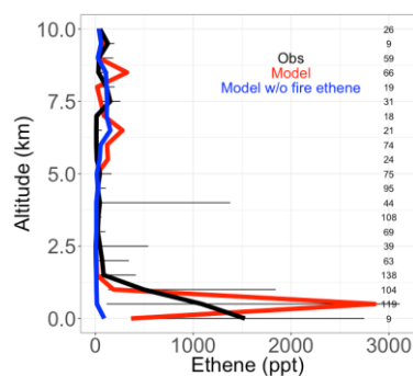
Fig 4. Median vertical profiles of binned ethene mixing ratios, including observed (black), simulated (red), and simulated in a sensitivity model run without fire ethene emissions (blue) during the boreal part of the ARCTAS campaign. Horizontal bars show the 25th–75th percentile range of measurements in each vertical 0.5-km bin. The number of observations in each vertical bin is shown on the right side of each panel.
