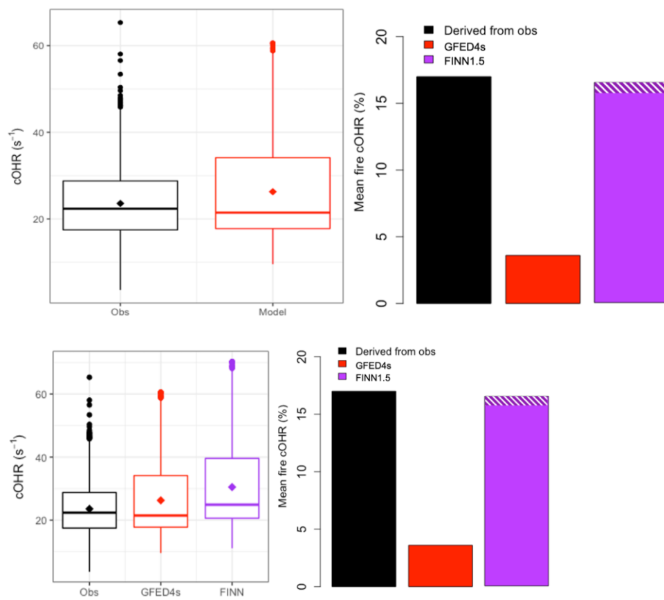
Figure 5. (Left) Boxplots of cOHR during the October 2018 and September 2019 measurement periods at ATTO with observations in black and the model in red with medians shown as a horizontal line and means as diamonds. (Right) The mean percentage contribution from fires during the same time period to cOHR with that derived from observations in black, the model with GFED4s in red, and a simulation using scaled-up FINN1.5 in purple. The white hatching on the FINN1.5 simulation indicates the increase in percentage contribution due to of new EFs and chemistry.
