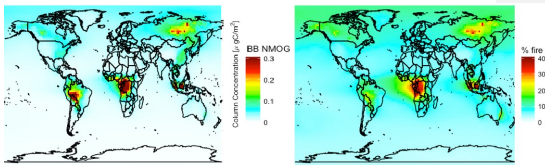
Figure 7. 2019 annual mean simulated (Left) NMOG total column concentrations from fires and (Right) percent contribution of NMOG total column concentrations from fires
