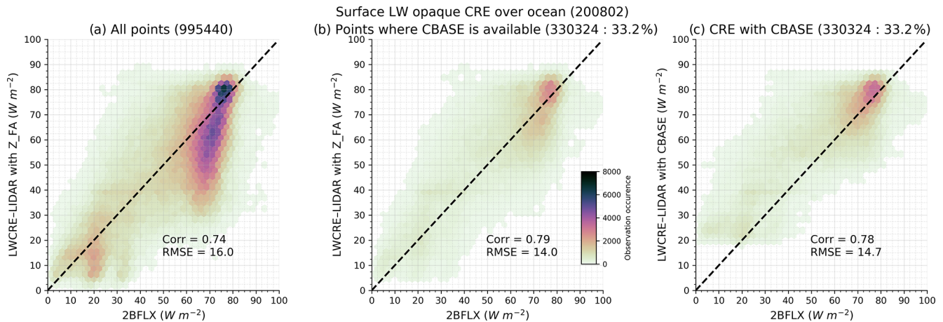
Figure 16. Surface LW CRE derived from LWCRE–LIDAR as a function of the one derived from 2BFLX. (a) Surface LWCRE–LIDAR ( y axis) computed using the altitude of full lidar attenuation (b) , same as (a) but containing only the subsample of CALIPSO profiles where cloud-base-height values are available from Mülmenstädt et al. (2018). (c) Same as (b) , but the surface LWCRE–LIDAR is computed using the cloud-base-height values from Mülmenstädt et al. (2018) instead of the altitude of lidar full attenuation. The color scale indicates the number of occurrences at 5 km resolution (footprint scale of CloudSat) over ocean in February 2008.
