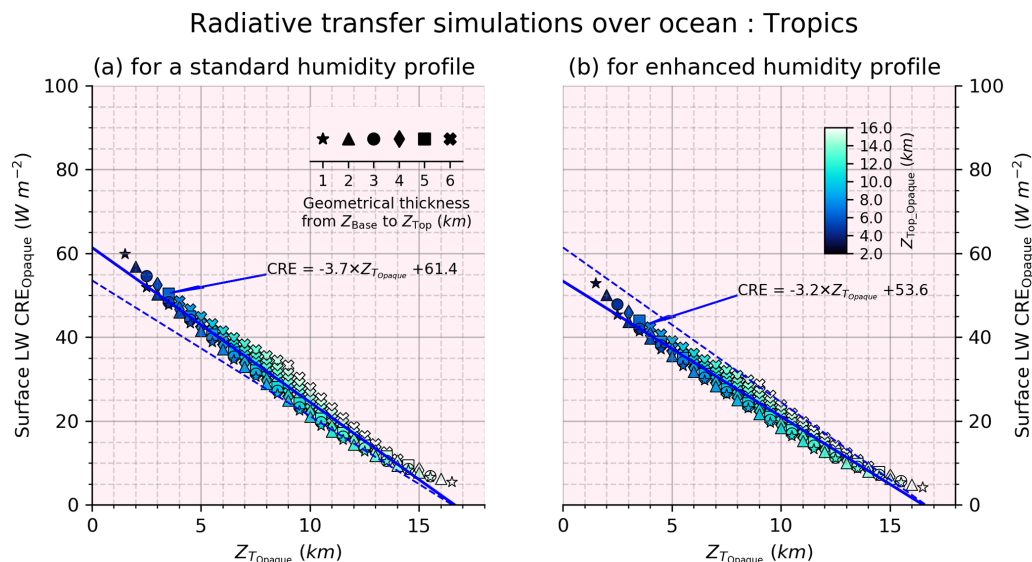
Figure 4. Same as Fig. 3a for (a) a standard humidity profile and (b) an enhanced humidity profile, both in the tropics: [30^{\circ} S-30^{\circ} N] .
