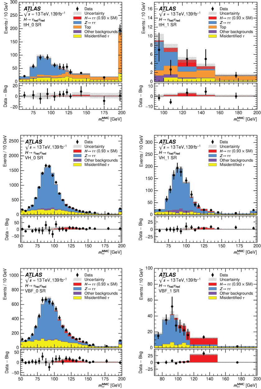
Figure 19. Distribution of the reconstructed \tau\tau invariant mass ( m_{\tau\tau}^{\text{MMC}} ) for all events in the t\bar{t}H , V(\text{had})H and VBF categories of the \tau_{\text{had}}\tau_{\text{had}} channel. The bottom panel shows the differences between the numbers of observed data events and expected background events (black points). The observed Higgs boson signal, corresponding to (\sigma \times B)/(\sigma \times B)_{\text{SM}} = 0.93 , is shown with a filled red histogram. Entries with values above the x -axis range are shown in the last bin of each distributions. The dashed band indicates the total uncertainty on the total predicted yields. The prediction for each sample is determined from the likelihood fit performed to measure the pp \rightarrow H \rightarrow \tau\tau cross-section.
