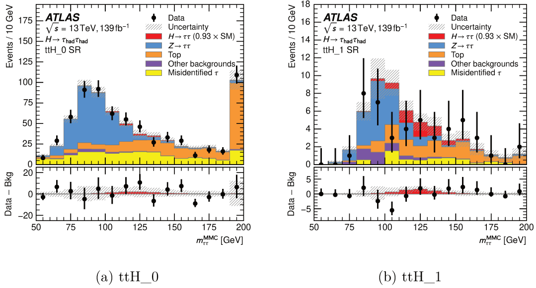
Figure 11. Distribution of the reconstructed \tau\tau invariant mass ( m_{\tau\tau}^{\text{MMC}} ) for all events in the (a) \text{ttH}_0 and (b) \text{ttH}_1 categories of the \tau_{\text{had}}\tau_{\text{had}} channel. The bottom panel shows the differences between the numbers of observed data events and expected background events (black points). The observed Higgs boson signal, corresponding to (\sigma \times B)/(\sigma \times B)_{\text{SM}} = 0.93 , is shown with a filled red histogram. Entries with values above the x -axis range are shown in the last bin of each distributions. The dashed band indicates the total uncertainty on the total predicted yields. The prediction for each sample is determined from the likelihood fit performed to measure the pp \rightarrow H \rightarrow \tau\tau cross-section.
