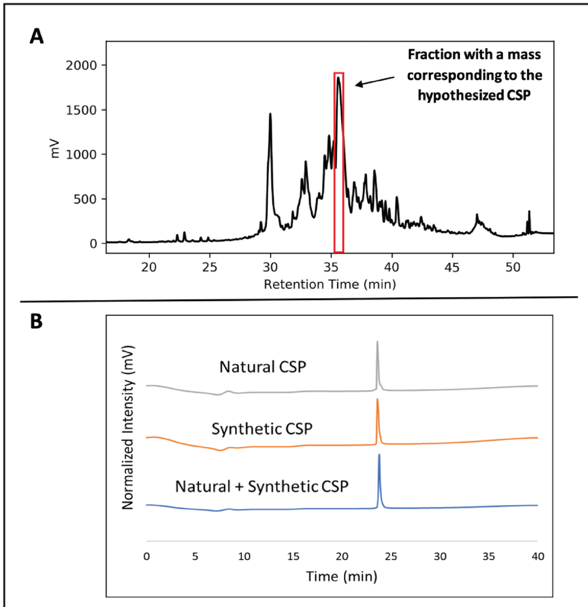
Figure 2. A) Preparative RP-HPLC trace of S. sinensis Forsyth1A spent supernatant following 30% ammonium sulfate precipitation. B) Analytical RP-HPLC trace comparing naturally isolated S. sinensis Forsyth1A CSP to synthetic CSP.
