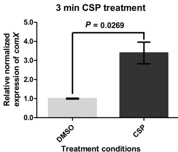
Figure 4. RT-qPCR results after 3-minute synthetic CSP treatment. Treatment with exogenous CSP for 3 minutes leads to activation of the comX gene. After a 3-minute incubation, stop solution was added to each sample to stop transcription. Data is normalized to expression of gyrB . The RT-qPCR experiment was conducted using two biological replicates for both the CSP and DMSO conditions.
