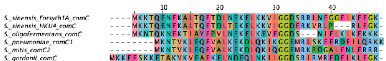
Figure 3. ClustalW alignment of the ComC proteins of several Mitis group streptococci. ComC is presented as a propeptide that is typically cleaved following the double-glycine motif to render the mature CSP signal.
