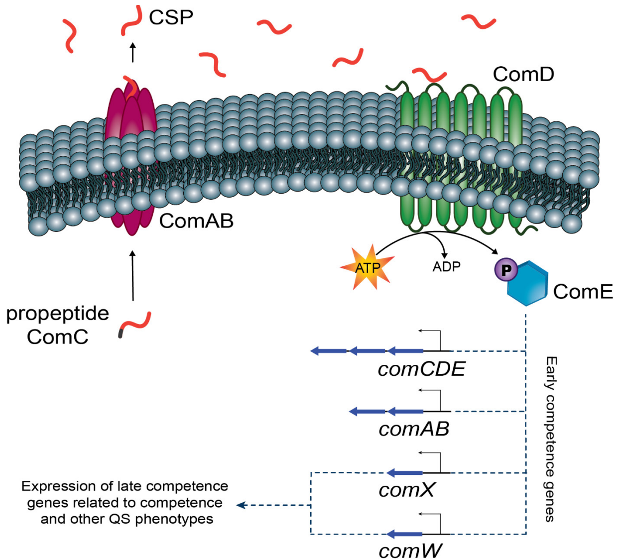
Figure 1. Depiction of the ComABCDE QS circuit regulating competence in Mitis group streptococci.
