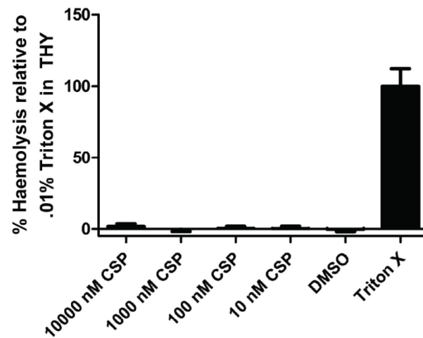
Figure 9. Effect of exogenous CSP on S. sinensis virulence factor production. The addition of exogenous CSP at varying concentrations does not significantly affect lysis of RBCs by S. sinensis . See the Supporting Information for full experimental details.
