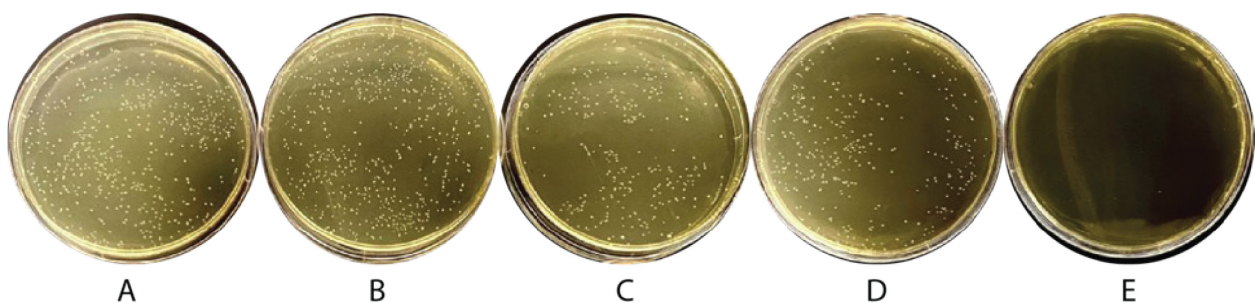
Figure 7. S. sinensis transformation assay. S. sinensis demonstrates dependence on the addition of exogenous synthetic CSP for the successful uptake of added plasmid (pDL278). The synthetic CSP was added at final concentrations of 10,000 nM (A), 1,000 nM (B), 100 nM (C), and 10 nM (D). The control includes no exogenous CSP (E). See Materials and Methods for full experimental details.
