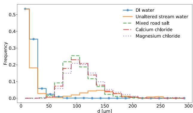
Figure 2. Volume-weighted normalized particle size distribution across different experiments at equilibrium at the turbulent shear rate of 35 \text{ s}^{-1} .
