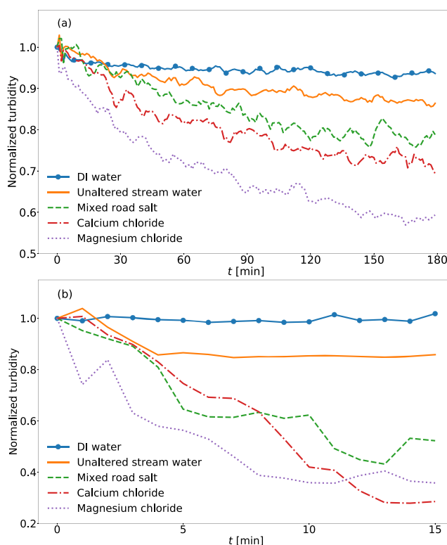
Figure 3. Time series of normalized turbidity at (a) turbulent shear rate of 20 \text{s}^{-1} and (b) stagnant water.
