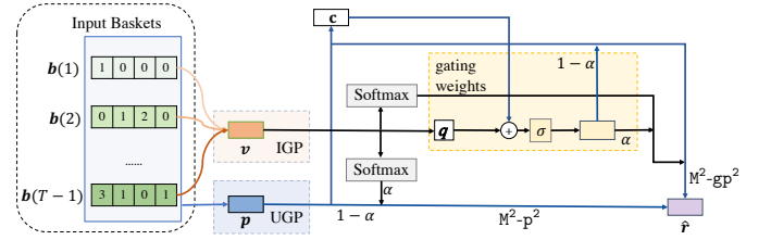
Fig. 1: M^2-p^2 and M^2-gp^2 Model Architectures
