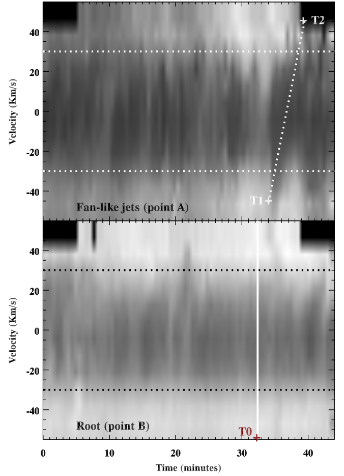
Figure 3. Temporal evolution of stacked H\alpha intensity from the blue wing to the red wing for point A on the path of the fan-like jets (top panel) and point B of the root (bottom panel). Different wavelengths along the vertical axis have been transformed into Doppler velocity, and the ones of \pm 30 \text{ km s}^{-1} are annotated with dotted horizontal lines for reference. The oblique dotted line in the top panel demonstrates the same jet event, and the white plus signs at the two ends mark the same times (T1 and T2) as demonstrated in Figure 2. Both the vertical white line and the red plus sign in the bottom panel show the time (T0) when the intensity profile of the root is displayed in Figure 4. Dark blocks at the corners exist owing to the missing observations at the H\alpha far wing in red.
