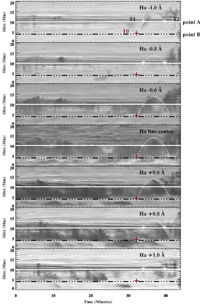
Figure 2. Time–distance plots that sample the recurrent fan-like jets along the blue curve in Figure 1 are displayed with a time range from 17:00 UT to 17:44 UT. Evolution in the wavelengths from H\alpha - 1.0 \text{ \AA} to H\alpha + 1.0 \text{ \AA} is shown from top to bottom. One jet event has been selected and outlined with white dotted parabolic lines. Points A and B, which are annotated with a white line and black dashed–dotted line, are selected to represent a point in the jet and the root, respectively. The white plus signs in the top and bottom panels show the times (T1 and T2) when upflow and downflow, which are mainly observed in H\alpha \pm 0.8 \text{ \AA} and \pm 1.0 \text{ \AA} , are passing through point A, respectively. The red plus sign in all panels shows the time (T0) when the intensity profile of the selected jet event is investigated later. Examples of the intensity evolution at points A and B of H\alpha from the blue wing to the red wing with a wavelength step of 0.2 \text{ \AA} are stacked and displayed in Figure 3.
