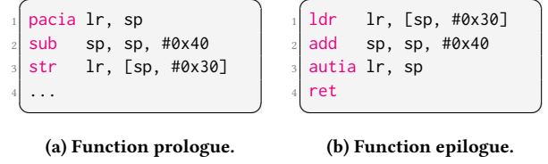
Figure 2: Stack protection using ARM Pointer Authentication.
