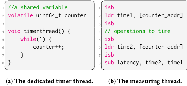
Figure 4: The multi-thread timer.
