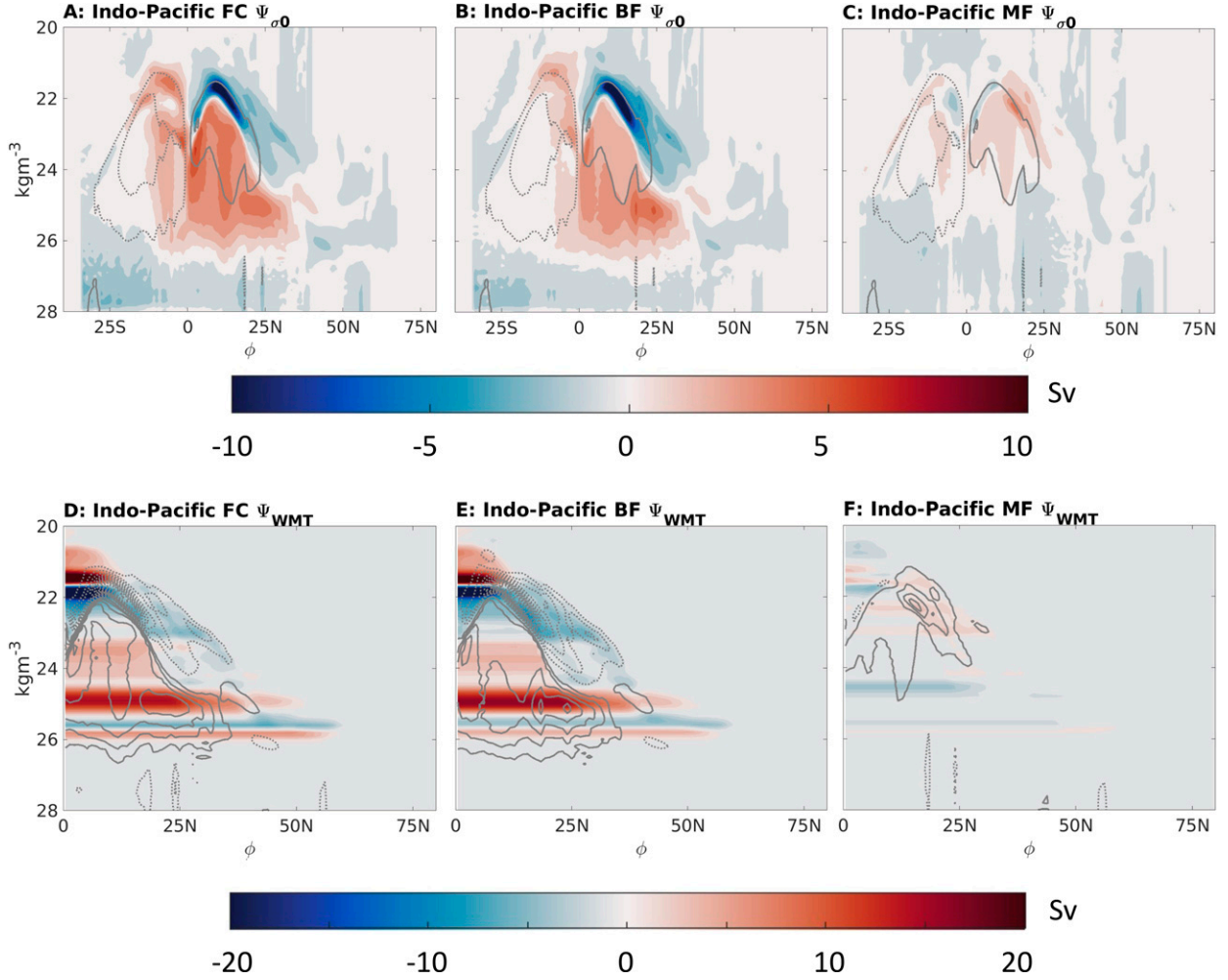
FIG. 9. (top) Indo-Pacific \Psi_{\sigma_0} response for (a) FC, (b) BF, and (c) MF as colored contours every 1 Sv. The time average of the unperturbed Indo-Pacific \Psi_{\sigma_0} in the control climate, Clim1, is given as gray contours of 10 Sv. (bottom) Indo-Pacific \Psi_{\text{WMT}} response for (d) FC, (e) BF, and (f) MF as colored contours every 1 Sv. The corresponding Indo-Pacific \Psi_{\sigma_0} response (colors from top row) is overlain as gray contours of 1 Sv.
