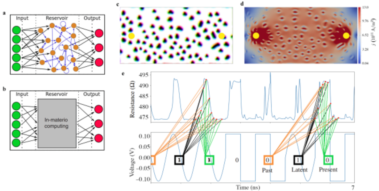
Fig. 12. Schematics of a recurrent neural network and b a material-based reservoir [205]. c Simulation of skyrmion reservoir. Locations of green and red circles refer to input and output contacts, respectively [205]. d Current density distribution across the skyrmion network shown in c after application of a voltage to the electrical nanocontacts represented by the yellow circles [205]. e Illustration of time-dependent training and operation of the output layer. The measured resistance values are summed by three different weights trained for recognizing either the present pulse, the latent pulse, or the past pulse [205].
