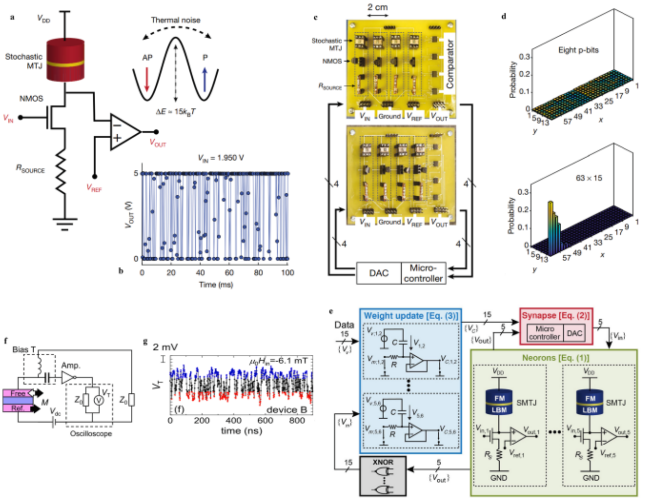
Fig. 9. a A probabilistic bit formed by a stochastic magnetic tunnel junction (MTJ) with a resistor, an NMOS transistor and a comparator. The energy profile between the parallel (P) and antiparallel (AP) states of the magnetization orientation of the stochastic MTJ is also shown [49]. b Time snapshots of the output signal V_{OUT} from the comparator for the input V_{IN} = 1.950 V, showing the fluctuation of the tunneling magnetoresistance induced by the fluctuation of the MTJ magnetization [49]. c A photograph of a probabilistic circuit composed of 8 stochastic MTJs. A microcontroller and a data acquisition (DAC) are interconnected for signal readout and weight implementation [49]. d The uncorrelated (top) and correlated (bottom) state of the circuit for integer factorization of 945 = 63 \times 15 . More than 2,000 sampling points are collected for statistics [49]. e Block diagram of the probabilistic learning circuit. \{V_{in}\} are input voltages to NMOS. \{V_{out}\} are output voltages from comparators. \{V_U\} are weight voltages. \{V_C\} are capacitor voltages. \{V_m\} are correlation voltages between probabilistic MTJs. \{V_v\} are data distribution correlation voltages. The RC network was used to model the Boltzmann-machine learning algorithm [48]. f Circuit configuration of the random telegraph noise (RTN) measurements of an in-plane MTJ [46]. g Time snapshots of the output signal V_T , showing a relaxation time of 8 ns of the in-plane MTJ [46].
