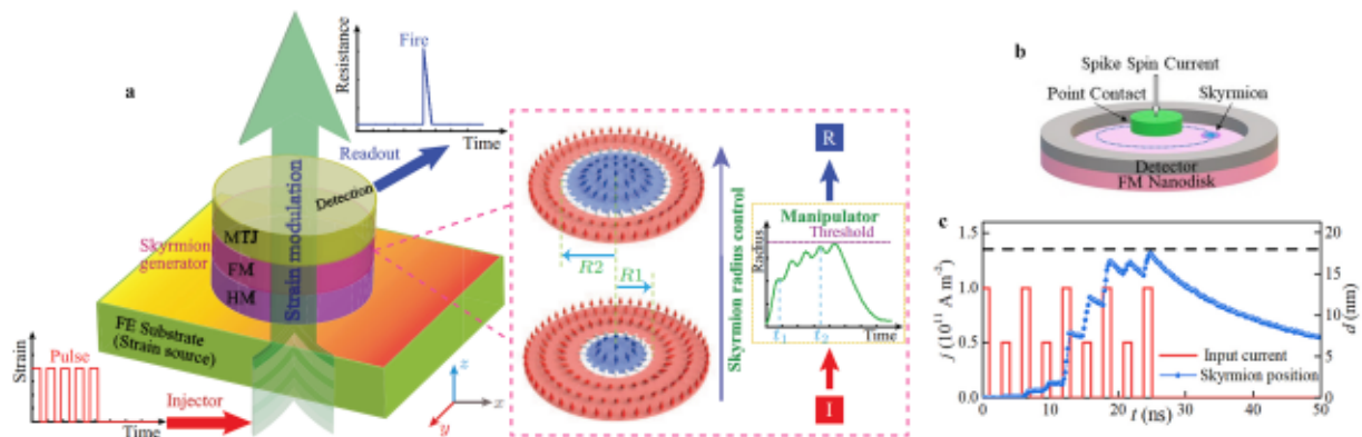
Fig. 7. a Illustration of a spiking neuron device that consists of a skyrmion generator, a magnetic tunnel junction (MTJ) detector, and an external strain source with pulsed modulation. Schematic of the variation in the skyrmion radius over time is illustrated in the inset. The skyrmion size increases under voltage pulses due to the modification of the PMA and returns back to its original size in the presence of the bias voltage [227]. b Schematic of a skyrmion-based spiking neuron consisting of a nanoscale point-contact, a skyrmion-based spin-torque nano-oscillator (STNO) and a ring-shaped electrode [228]. c Time-dependent skyrmion position under the influence of a nonuniform square wave spike current with frequency of 0.5 GHz. The current is applied through the center nanorod and flows radially towards the ring-shaped electrode. The radial distribution of the current causes the skyrmion to move circularly such that the radius of motion serves as the membrane potential [228].
