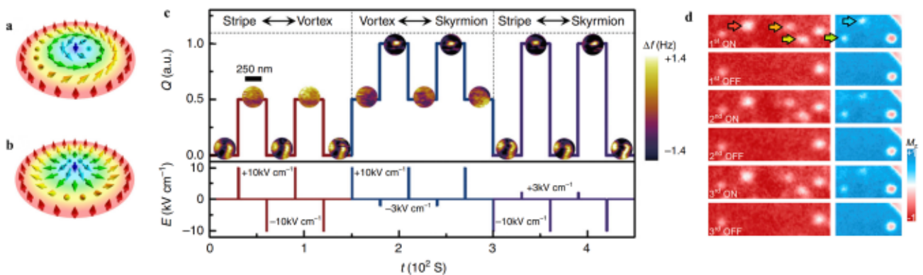
Fig. 1. a Bloch-type and b Néel-type skyrmion configurations [59]. c Switching of individual skyrmions in a nanodot with a diameter of 350 nm induced by a pulsed electric field E . The top panel shows fluctuations in the topological number Q over time in response to an applied 1 ms voltage pulse (bottom panel). The different magnetic domains included here are the skyrmion ( Q = 1 ), vortex ( Q = 0.5 ), and stripe ( Q = 0 ). Switching between these domains is illustrated by magnetic force microscope (MFM) images and quantified by the energy required to make the transition [110]. d Experimental results of reversible writing/deleting of magnetic skyrmions in a Ni/Co/Pd/W(110) thin film via chemisorption and desorption of hydrogen gas. An ON cycle involves supplying a dose of hydrogen gas to write skyrmions. An OFF cycle allows sufficient time for spontaneous hydrogen desorption and recovery of the magnetization to the initial state. Red and blue regions refer to the evolution of the perpendicular magnetization of the sample [115].
