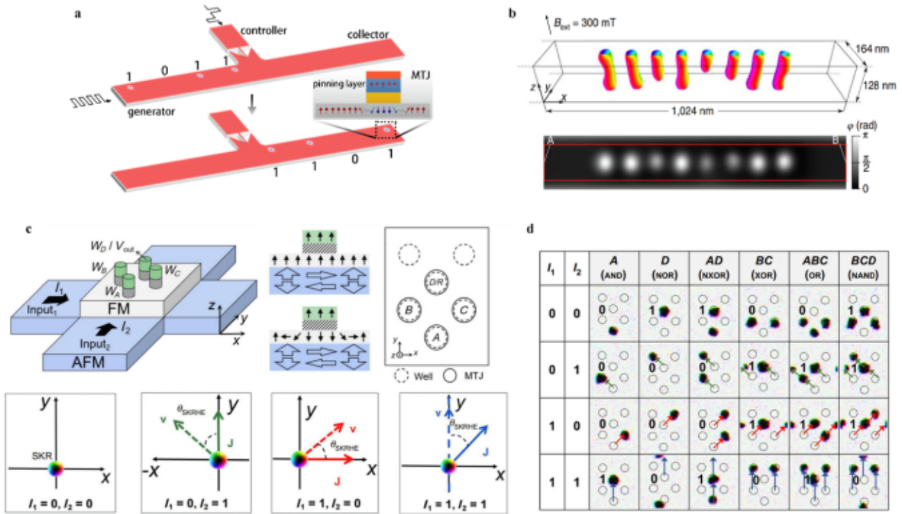
Fig. 3. a Schematic of a three-terminal racetrack memory device. The generator creates the skyrmion which is then detected at the collector. The presence or absence of a skyrmion is used to encode a bit 1 or 0, respectively. A voltage pulse can be applied in the controller terminal to create or delete a skyrmion, thereby enabling the modification of the skyrmion information in a controlled manner. This figure shows a correction of the bitstream from “1101” to “1011” which is then detected at the collector [145]. b Top: Micromagnetic simulation results for a chain of skyrmions and chiral bobs in the presence of a perpendicular magnetic field in a thin strip of FeGe. Bottom: Phase shift of an electron beam \varphi calculated for each configuration in the Top image. The phase shift can be detected by means of quantitative off-axis electron holography in a transmission electron microscope (TEM) [175]. c Top left: Diagram of ferromagnetic-antiferromagnetic (FM-AFM) bilayer device. Identical currents I_1 and I_2 serve as input signals to the AFM layer. Magnetic tunnel junctions (MTJs) A-D write the skyrmions and read the output voltage. Top center: MTJ spin configurations with the presence (top) and absence (bottom) of a skyrmion. Top right: Aerial view of MTJs (solid circles) and pinning centers (dashed circles). Bottom: Skyrmion motion in the FM layer under different current densities J and their resulting velocities v . The skyrmion motion (dashed arrows) deviates from the current direction (solid-colored arrows) due to the skyrmion Hall angle [181]. d Simulation results of various logic operations performed using the device structure in c. Skyrmions are positioned using pinning sites and move in response to applied input currents with trajectories indicated by the colored arrows [181].
