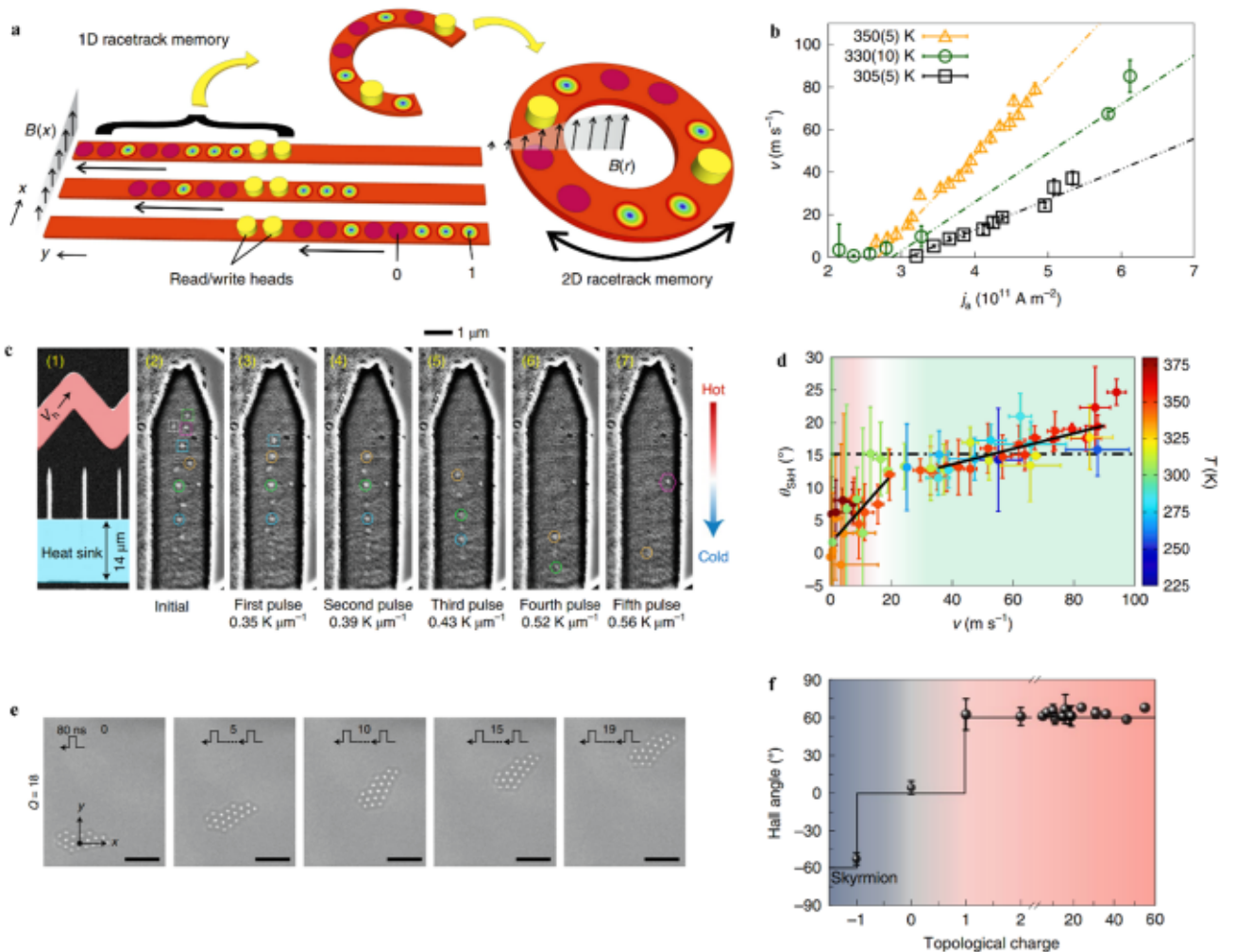
Fig. 2. a Schematic of a racetrack memory concept. In one-dimensional racetrack memory, the presence or absence of skyrmions is used to encode bits 1 or 0, respectively, as the skyrmion stream moves across the track past read/write heads. Further degrees of freedom can be accessed by bending these strips into circles to create two-dimensional racetrack memory. Motion of skyrmions in this disk can be achieved by an external applied field gradient B(r) [86]. b Plot of skyrmion velocity as a function of current density at several sample temperatures. Variation in the slopes stems from spin-orbit torque (SOT). The results are obtained in a [\text{Pt} (2.7 \text{ nm})/\text{CoFeB}(0.86 \text{ nm})/\text{MgO}(1.5 \text{ nm})]_{15} multilayer stack [153]. c Illustration of thermally induced skyrmion motion. (1) Scanning electron microscopy (SEM) image of the device. 500 ms pulse voltages V_h are applied to the Ta/Pt heater. A temperature gradient is created across the [\text{Ta}/\text{CoFeB}/\text{MgO}]_{15} nanowires between the heater and the heat sink via thermal dissipation in the insulating \text{Si}_3\text{N}_4 thin layer underneath. (2)–(7) Unidirectional diffusion of skyrmions observed from hot to cold regions in response to 500 ms pulse voltages V_h . Here, several different dynamics are observed including pinned skyrmions, skyrmion annihilation and long-range skyrmion diffusion [93]. d Skyrmion Hall angle (SHA) \theta_{\text{SKH}} as a function of skyrmion velocity at various temperatures in the same structures as b. Two distinct regions are observed. The creep regime (red region) is characterized by a steep increase in the SHA with velocity while in the flow regime (green region) the slope is notably smaller. The theoretical disorder-free SHA for skyrmions is indicated by the black dashed line [153]. e Lorentz transmission electron microscopy (TEM) images of current-induced motion of skyrmion bundles with Q = 18 . A series of 80 ns pulses are applied in the -x direction at a perpendicular field of 100 mT. As expected by the skyrmion Hall effect, the bundles move in the +x direction with a notable transverse motion in the y direction [164]. f Plot of SHA as a function of the topological charge Q of skyrmion bundles. It is evident that the sign of the Hall angle is dependent on the sign of the topological charge. Furthermore, the Hall angle is seemingly independent of the applied current density, external field, and Q [164].
