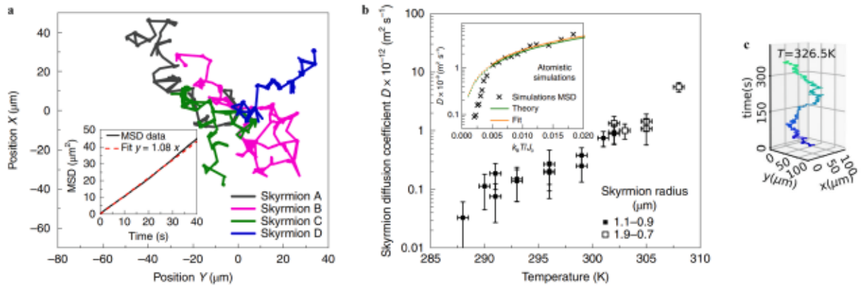
Fig. 4. a Position of four different skyrmions at room temperature in a low-pinning Ta/CoFeB/Ta/MgO/Ta multilayer measured using magneto-optic Kerr effect (MOKE) microscopy. The inset illustrates the time-averaged mean squared displacement (MSD) of the data [92]. b Semilogarithmic plots of the observed and simulation-based (inset) skyrmion diffusion constant as a function of temperature. Strong temperature dependence in the low temperature regime is predicted by the simulation, followed by quasi-free diffusion restored as the temperature is increased. Data points are averaged over measuring several skyrmions [92]. c Time-dependent trajectory of an isolated skyrmion with Q = -1 in a Ta/CoFeB/TaO x multilayer at 326.5 K. The Brownian gyromotion is observed [192].
