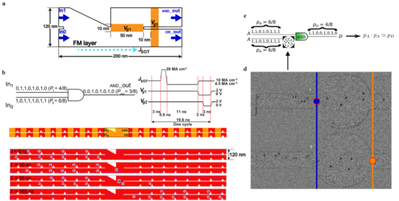
Fig. 11. a Skyrmion-based AND/OR logic gates with two input and output tracks. The electrode gates V_{g1} and V_{g2} are used to control skyrmion motion by the VCMA effect [243]. b Top left: Multiplication operation using AND gate. Top right: Contour of driving current density and electrode voltages over one cycle. Center: Schematic of skyrmion stochastic multiplier. The white notches separate the top and bottom tracks into eight regions. Bottom: Magnetization configuration of schematic in center diagram at various timestamps. At t = 0 ns, the input probabilities are 4/8 and 6/8 in the top input and bottom input tracks, respectively. After the application of a current density, the AND track correctly yields the multiplied probability of 3/8 , or “00101010” as a binary sequence [243]. c Schematic of a stochastic computing device using AND gate. One input signal is first reshuffled using the reshuffler device in d and becomes uncorrelated while retaining the same probability values [91]. d Skyrmion reshuffler device operation in a Pt 95 Ir 5 /Fe/Pd thin film. Skyrmions are nucleated by applied currents and their motion across the blue and orange lines dictates the input and output signals, respectively, in terms of bits “0” and “1” [92].
