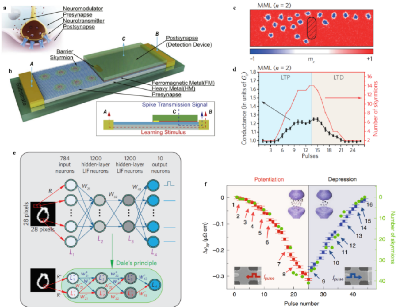
Fig. 8. a Illustration of biological synapse with relevant parts labeled [232]. b Design of a skyrmion synapse. Neuromodulator is modeled by a learning stimulus that passes through the heavy-metal (HM) layer from terminal A to B. This stimulus can either drive the skyrmions into the post-synapse region, in which case the synaptic weight increases, or back into the presynaptic region, by which the synaptic weight would decrease. This resembles the biological processes of potentiation and depression, respectively. Terminal C measures the synaptic weight [232]. c Results of micromagnetic simulations of a skyrmion synapse with colors representing the direction of magnetization in a [\text{HM}/\text{FM}/\text{HM}]_n stack at room temperature (where n = 2 ). The rounded rectangular barrier is illustrated, separating the pre- and postsynaptic regions [231]. d Plot showing the variation in conductance of the sample (black data) relative to the number of skyrmions in the post-synapse region (red data) [231]. e Schematic of skyrmion-based deep ANN including input neurons, two sets of hidden-layer LIF neurons, output neurons, and synaptic weights ( W_{ij} ) used to learn the handwritten pattern provided as input [231]. f Measured Hall resistivity change and calculated skyrmion number as a function of injected pulse number in [\text{Pt} (3 \text{ nm})/\text{Gd}_{24}\text{Fe}_{66.6}\text{Co}_{9.4} (9 \text{ nm})/\text{MgO} (1 \text{ nm})]_{20} ferrimagnetic multilayer stacks. The red/blue symbols and colored areas correspond to resistivity changes (left axis) during potentiation and depression, respectively. Green symbols indicate the number of skyrmions (right axis). Insets illustrate the direction of charge current pulses [234].
