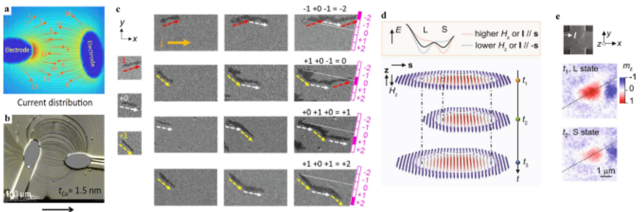
Fig. 5. Local dynamics of skyrmions. a Simulation of electric current distribution in a cobalt film using finite element modeling. b Emergence of magnetic strip domains in Ta/Pt/Co/Ta multilayer after applying a voltage pulse. Yellow lines indicate electric current distribution calculated in a [206]. c Addition operations achieved through chiral stripe domain elongation in W/CoFeB/MgO/Ta films in response to applied magnetic fields and current pulses. Each operation is carried out under a specific set of magnetic fields together with x-axis current pulses of 50 ms with a constant current density. The half-skyrmion exhibits distinct trajectories marked by red (+1), white (0), and yellow (-1) arrows under different sets of magnetic fields. The results of the operations, indicated by the termination of the stripe, are shown in pink [207]. d Schematic illustrating the fluctuation dynamics of skyrmions between large-skyrmion (L) and small-skyrmion (S) states over time as a result of interactions with local pinning centers. The energy barrier that exists between these two states, illustrated in the top panel, can be further tuned by the applied field and current. e MOKE images of an isolated skyrmion in the L and S states measured in a Ta/CoFeB/MgO/TaO x multilayer patterned into a Hall cross structure [76].
