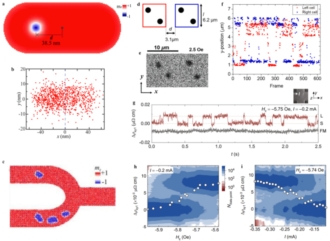
Fig. 10. a Top view of a true random number generator (TRNG) device based on the Brownian motion of a skyrmion with magnetization configuration of the m_z component in a heavy-metal/ferromagnetic (HM/FM) multilayer stack [191]. b Scatter plot of skyrmion position over a time interval of 1000 ns with 1 ns between consecutive data points [191]. c Top view of a TRNG device based on antiferromagnetic skyrmions [244]. d Schematic and e MOKE images of a skyrmion cellular automaton consisting of two adjacent square cells, each hosting two skyrmions [195]. f Time-dependent position of the two skyrmions closest to the gap, one in each of the red and blue cells [195]. g Inset: a TRNG device using the local dynamics of a skyrmion with the Hall cross as a transducer for signal readout and processing. The relative Hall-resistivity \Delta\rho_{xy} fluctuates in time between \Delta\rho_{xy} \approx 0 and \Delta\rho_{xy} \approx 0.008 \mu\Omega \text{ cm} for a single skyrmion. This corresponds to a skyrmion-size fluctuation between the small (S)-skyrmion and large (L)-skyrmion configuration. The signal for a saturated ferromagnetic (FM) state is also shown [76]. h Density of data points for the \Delta\rho_{xy} as a function of an applied field H_x at a fixed applied current of I = -0.2 \text{ mA} . White dots represent time-averaged resistivities. [76]. i Density of data points for the \Delta\rho_{xy} as a function of applied current I at a constant magnetic field of H_x = -5.74 \text{ Oe} [76].
