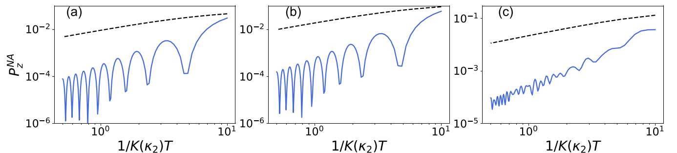
FIG. 9. Plots of P_z^{\text{NA}} vs 1/K(\kappa_2)T in a log-log scale for gates with dissipative (black dashed curves) and hard control (blue solid curves), which highlight that P_z^{\text{NA}} \propto 1/\kappa_2 T for dissipative gates while P_z^{\text{NA}} \propto 1/(KT)^2 for Kerr gates with hard control. (a) Z rotation. (b) ZZ rotation. (c) CX gate.
