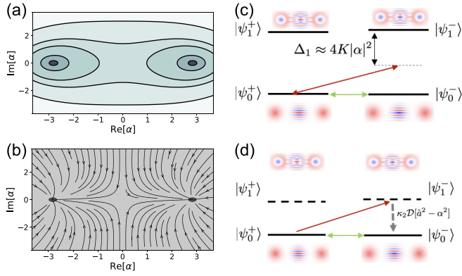
FIG. 1. (a) The semiclassical potential \langle \hat{H}_{\text{KPO}} \rangle of a Kerr cat in phase space. (b) The semiclassical dynamics of a dissipative cat in phase space. (c) and (d) Mechanism of the nonadiabatic errors during the z -axis rotation on (c) Kerr cats and (d) dissipative cats. |\psi_0^\pm\rangle, |\psi_1^\pm\rangle denote the first two pairs of eigenstates of \hat{H}_{\text{KPO}} with parity \pm , and the spacing between states in the vertical axis in (c) and (d) represents the energy gap and dissipative gap of the Kerr cat and the dissipative cat, respectively. For Kerr cats in (c), the nonadiabatic errors induced by the linear drive [\Omega(t)\hat{a} + \text{H.c.}] manifest in the form of off-resonant leakage. For dissipative cats in (d) with a dissipation gap, the linear drive induces decoherence within the cat-state manifold when combined with the engineered two-photon dissipation.
