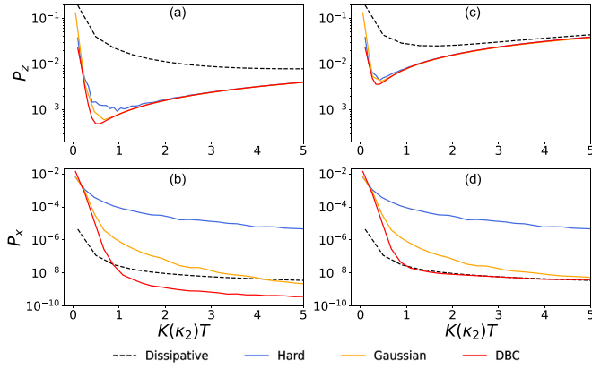
FIG. 3. The total Z and X error probabilities for the CX gate using different control schemes (same color scheme as Fig. 2) in the presence of photon loss. (a) and (b) \kappa_1/K(\kappa_2) = 5 \times 10^{-5} . (c) and (d) \kappa_1/K(\kappa_2) = 5 \times 10^{-4} . The gate time is in units of K(\kappa_2) for Kerr (dissipative) gates.
