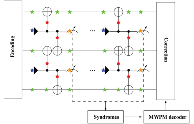
FIG. 4. The QEC circuit of the repetition cat. The potential faulty operations are the state preparation (blue), idling (green), CX gate (red), and measurement (orange). The measured syndromes are fed into the minimum weight perfect matching (MWPM) decoder to determine the errors.
