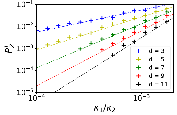
FIG. 11. Logical Z error probability of the logical CX gate encoded in a repetition cat using dissipative CX gates. The pluses are the MC simulation results, while the dashed lines are the fitting results P_Z^L = A[B\frac{\kappa_1}{\kappa_2}]^{\frac{d+1}{4}} . For this plot, \eta_T is set to 1, and the fitted coefficients are A = 0.16 , B = 352.1 .
