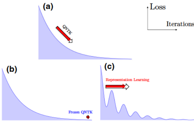
FIG. 1. An illustration of the QNTK theory. (a) The QNTK characterizes the gradient-descent dynamics in the variational quantum circuit. The quantum state modifies according to the QNTK prediction. (b) Around the end of the training, the QNTK is frozen and almost a constant. (c) The gradient-descent dynamics could be highly nonlinear, and the QNTK is running during gradient descent, which is a property of representation learning.
