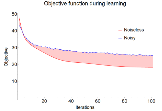
FIG. 5. Convergence of the objective function during gradient descent. Here we compare the ideal and noisy cases, labeled by red or blue, respectively.
