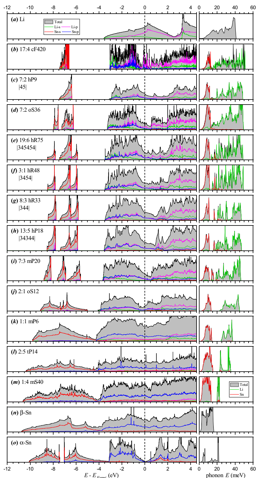
Fig. 8 Electron and phonon DOS calculated with the DFT for known and predicted ambient-pressure Li-Sn phases. The colored lines illustrate the DOS projected onto s and p orbitals for electrons (left panels) or onto Li and Sn atoms for phonons (right panels).
