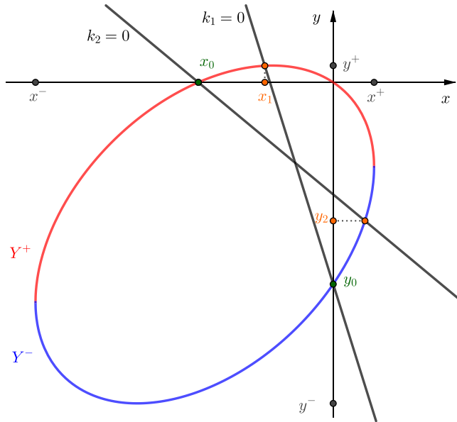
Fig. 4. The ellipse K = 0 , the function Y^- in blue, the function Y^+ in red, the two lines k_1 = 0 and k_2 = 0 , the branch points x^\pm and y^\pm , the points x_0 and y_0 in green, and the points x_1 and y_2 in orange. This figure is drawn for the following parameters: \mu_1 = 2 , \mu_2 = 3 , \rho = -0.4 , r_1 = 2 , r_2 = 4 . (For a colored version of this figure, please see the electronic version of this article.).
