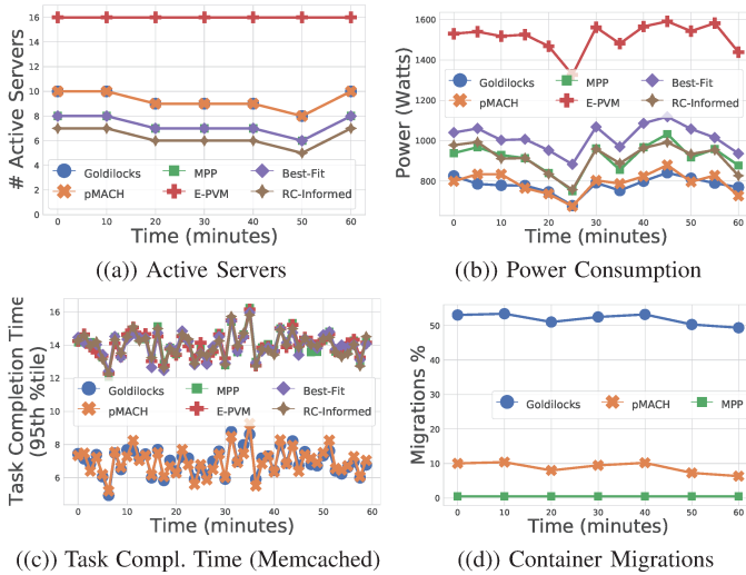
Fig. 9: Scheduling quality with a testbed containing 16 servers.
