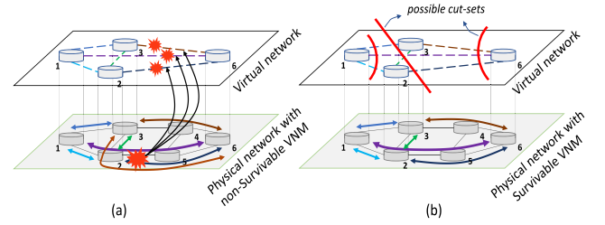
Fig. 2. (a) Non-survivable VNM and (b) SVN of a 4-node VN of 6 virtual links onto a 6-node sample physical network topology.
