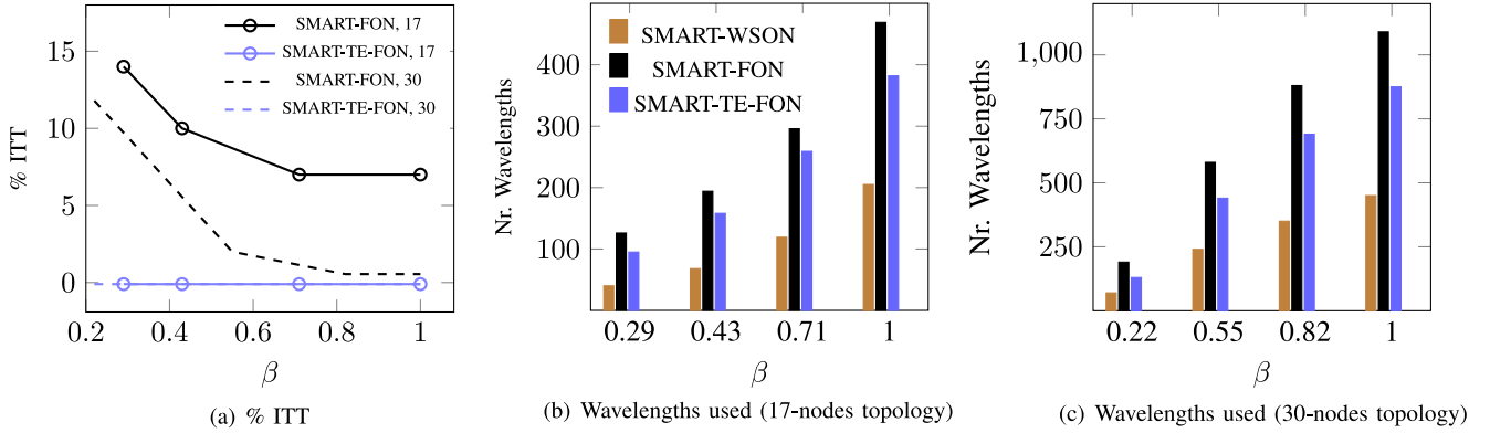
Fig. 8. %ITT and Nr. Wavelengths for the different network scenarios as a function of \beta for two the 17-nodes (referred to as 17 in legend of (a)) and the 30-nodes (30 in legend of (a)) physical topologies.
