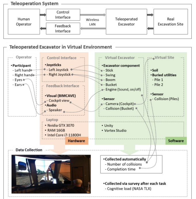
Figure 3. Human-robot interaction in a virtual environment
