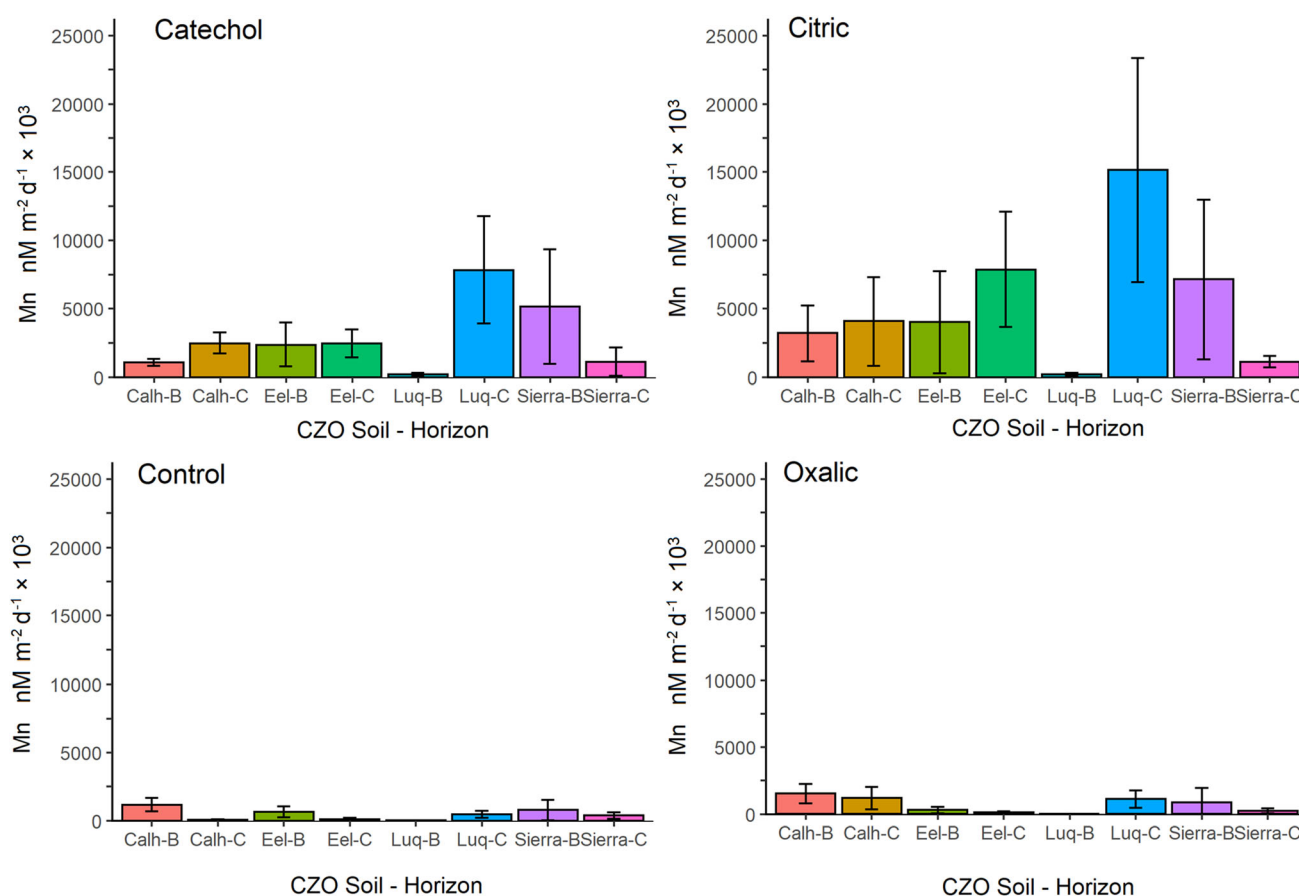
Fig. 4 Manganese dissolution rates normalized to soil surface area for B and C horizons at Calhoun, Eel River, Luquillo, and Southern Sierra CZOs under catechol, citric acid, oxalic acid, and control (HCl only) at pH 4.5 over 14 days. Samples were completed in triplicate per batch and repeated four times
