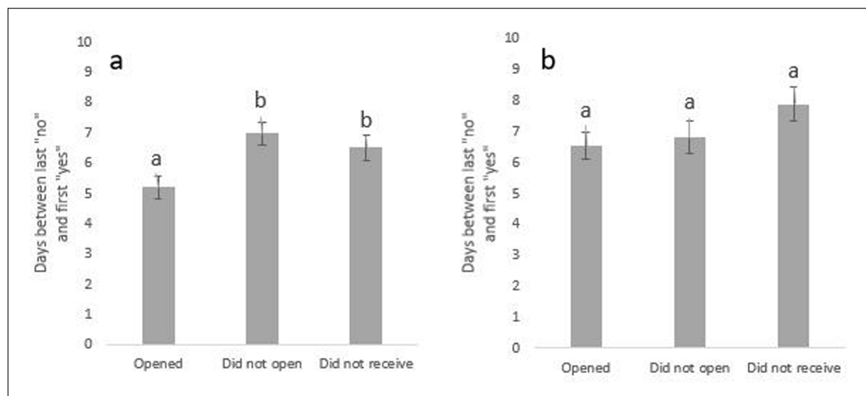
Figure 2 Precision in reports of phenological transitions contributed by Nature's Notebook observers that received and opened, received but did not open, and did not receive email-based messages, shown as the number of days between when the observer reported a "no" and when they first reported "yes" to (a) leaf-out and to (b) open flowers. Error bars represent two standard deviations. Levels not connected by the same letter are significantly different.
