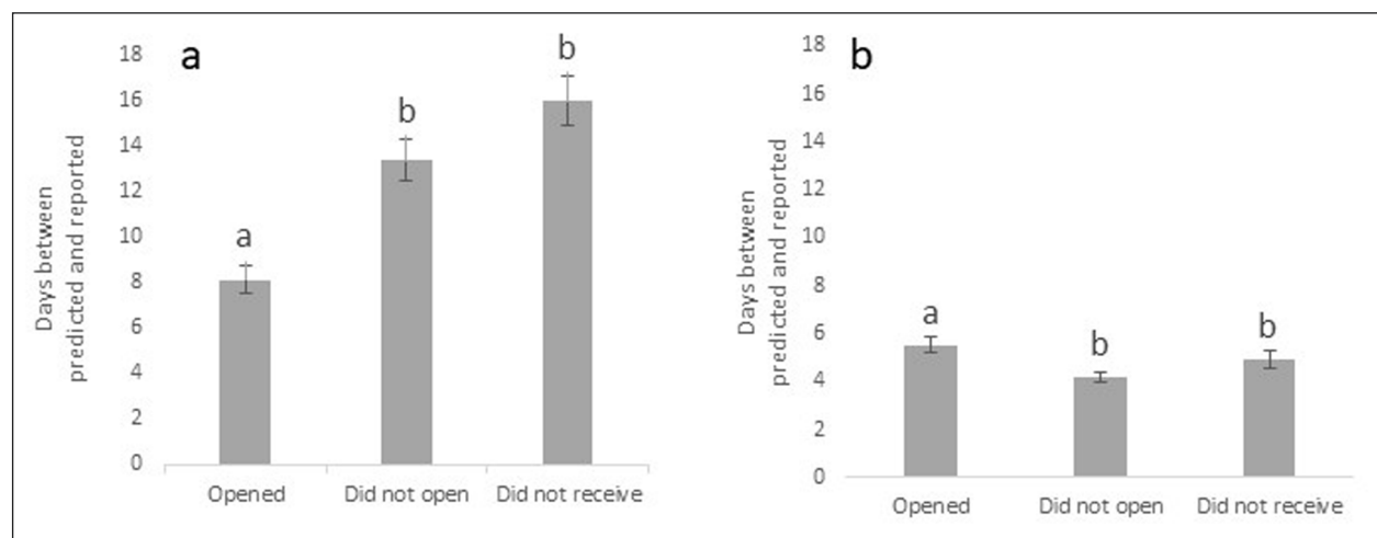
Figure 1 Accuracy in reports of phenological transitions contributed by Nature's Notebook observers that received and opened, received but did not open, and did not receive email-based messages, shown as the number of days between when (a) leaf-out and (b) bloom was predicted to occur and when it was reported to occur in lilacs. Error bars represent two standard deviations. Levels not connected by the same letter are significantly different.
