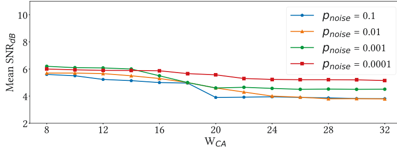
Fig. 9. The mean \text{SNR}_{\text{dB}} of CardiacWave with different settings of W_{\text{CA}} and p_{\text{noise}} .
