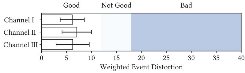
Fig. 13. The weighted event distortion of CardiacWave.
