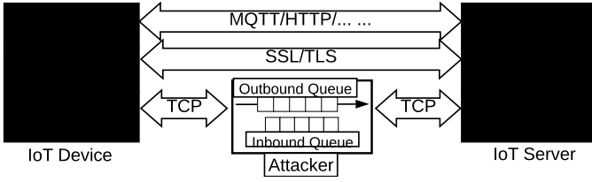
Fig. 2: Delaying IoT messages via a TCP hijacker.
