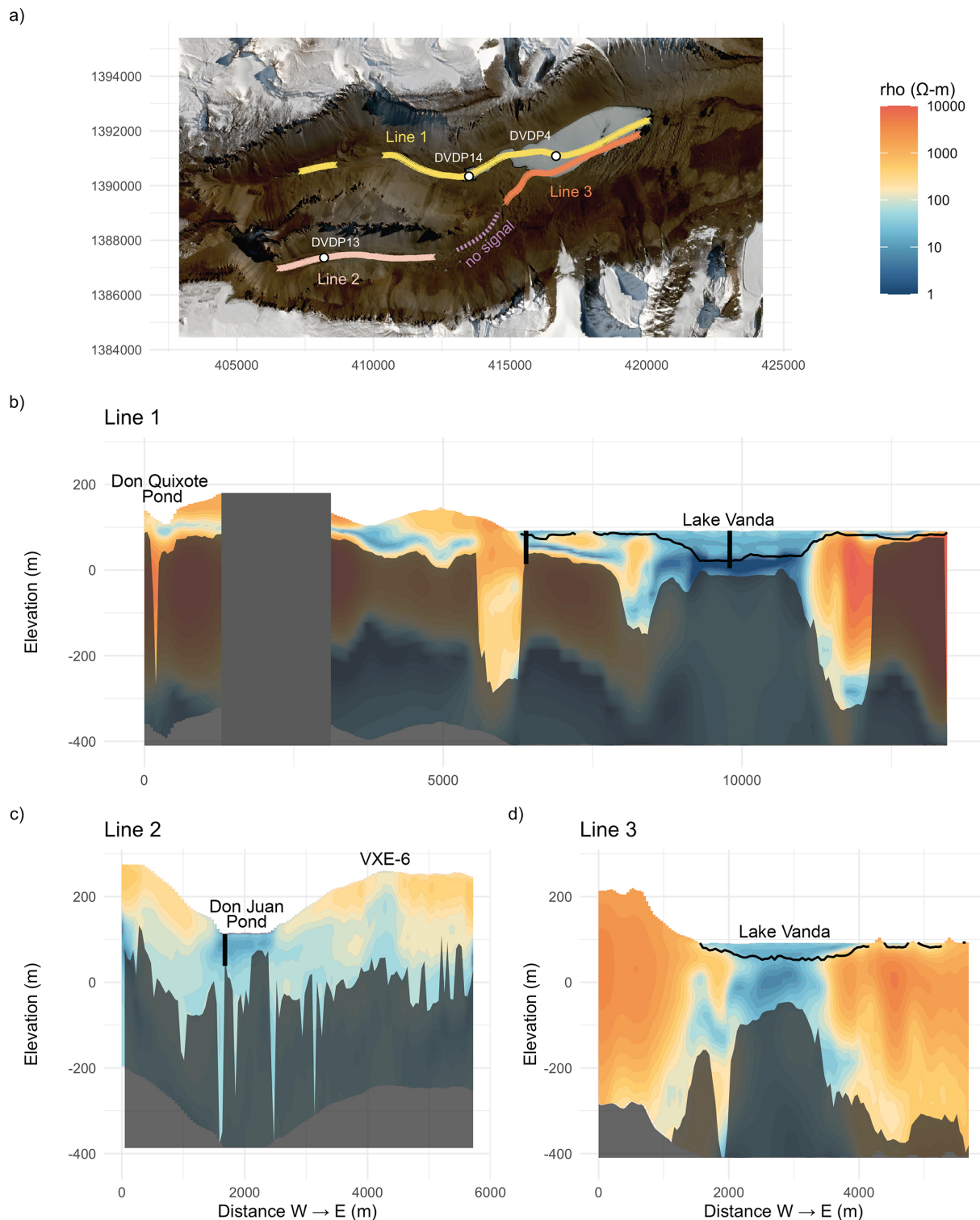
Figure 1. (a) AEM flight lines over the North Fork of Wright Valley and Lake Vanda (Line 1), over Don Juan Pond (Line 2), and over Lake Vanda towards the South Fork (Line 3). White circles show the locations of the DVDP boreholes. Coordinates are in UTM-58S. This contains modified Copernicus Sentinel data 2020. (b–d) Resistivity profiles of the three flight lines. The black line represents the sediment–water interface (bathymetry) of the Lake Vanda basin. Lower data are shaded beyond the depth of investigation. Black vertical rectangles show the approximate location and depth of the DVDP boreholes crossed by Lines 1 and 3.
