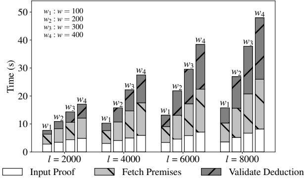
Figure 9: Verification time vs. refutation length. For different fixed refutation widths w , verification time is linear in the refutation’s length l . As the length grows, the increase in time of inputting proof is less than the increase for fetching premises and checking resolution. Furthermore, as length increases, the time for fetching premises and checking resolution dominates verification time.
