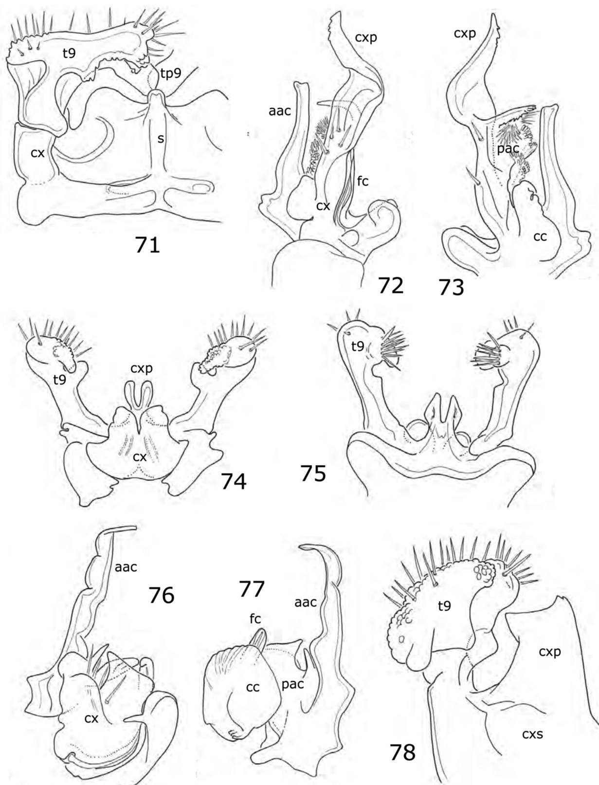
FIGURES 71–78. Striariid millipedes. 71. Right leg 9 of male Lamparia millicoma , n. gen., n.sp. , anterior view. Figs 72–75. Rampalia cheathamensis , n. gen. n. sp. 72. Right gonopod, lateral view. 73. Right gonopod, mesal view. 74. Male ninth legpair, anterior view. 75. Male ninth legpair, posterior view. Figs 76–78. Plaramia arcata , n. gen., n. sp. 76. Right gonopod, lateral view. 77. Right gonopod, mesal view. 78. Left leg 9 of male, anterior view. Abbreviations: aac , anterior angiocoxite; cc , colpocoxite; cxp , coxal process; cx , gonopod coxa; fc , flagellocoxite; pac , posterior angiocoxite; t9 , telopodite of ninth leg.
