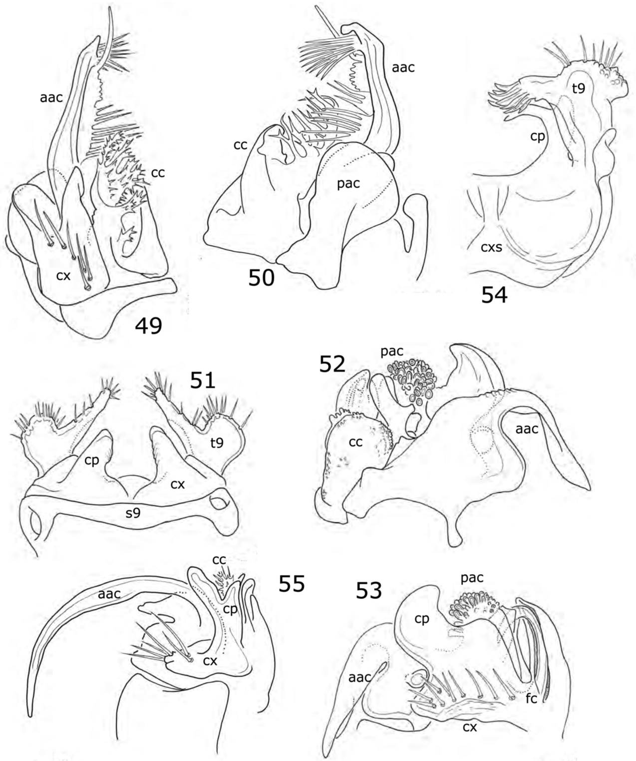
FIGURES 49–55. Striariid millipedes. Figs 49–51. Nototrisaria ornata , n. gen., n. sp. , right gonopod, lateral view. 50. Same, mesal view. 51. Legpair 9 of male, anterior view. Figs 52–54. Maraplia napa , n. gen., n. sp. 52. Right gonopod, mesal view. 53. Right gonopod, lateral view. 54. Right leg 9 of male, posterior view. 55. Right gonopod of Maraplia schusteri , n. gen., n. sp. , lateral view. Abbreviations: aac , anterior angiocoxite; cc , colpocoxite; cp , coxal process; cx , gonopod coxa; fc , flagellocoxite; pac , posterior angiocoxite; s9 , sternum of ninth legs; t9 , telopodite of ninth leg.
