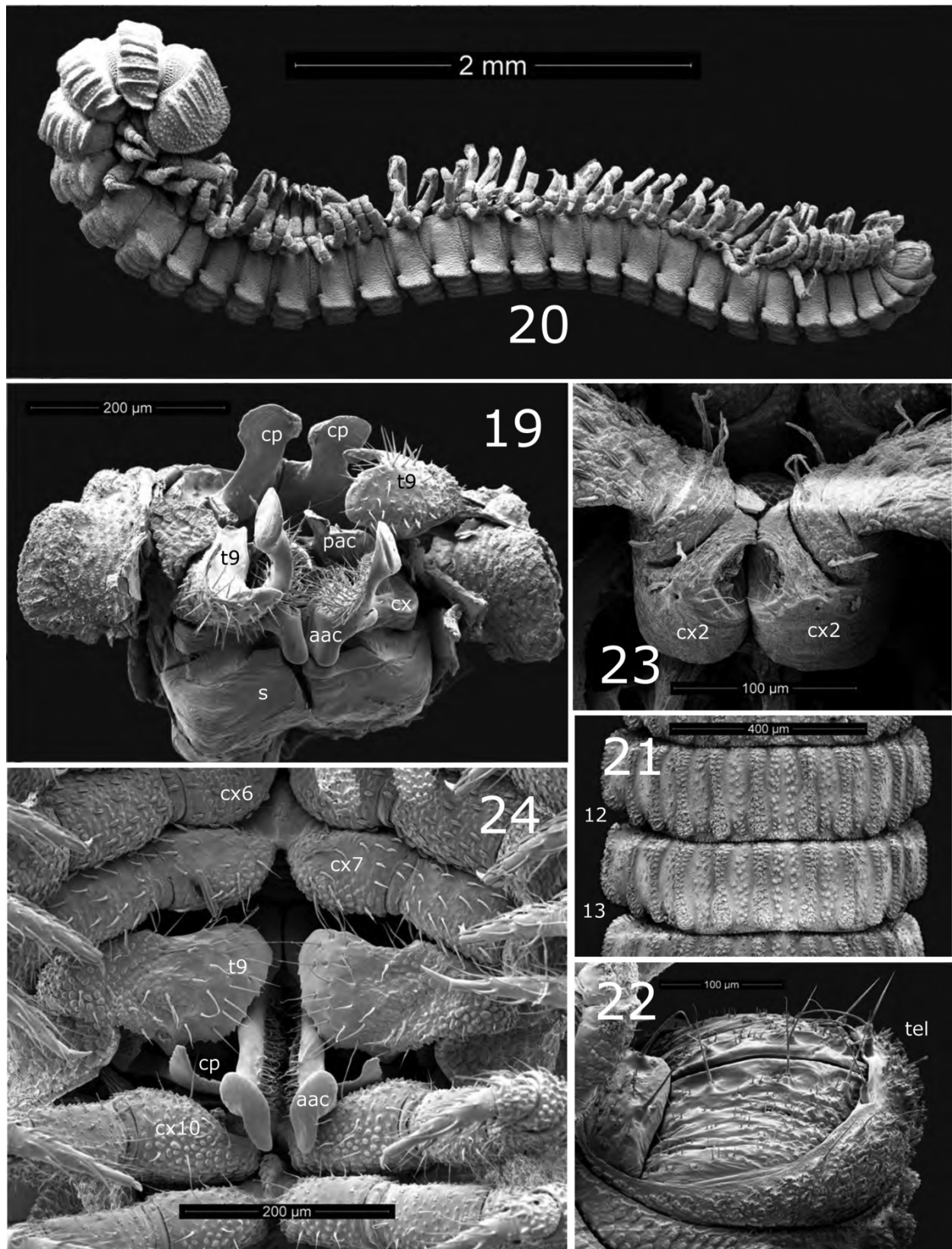
FIGURES 19–24. Striariid millipedes. 19. Gonopod, ninth legs, and ring 7 of Lamparia curryensis , n. gen., n. sp. , anteroventral view. Figs 20–24. Lamparia bentonensis , n. gen., n. sp. 20. Female, lateral view. 21. Rings 12 and 13 of male, dorsal view. 22. Telson, paraprocts and epiproct, ventral view. 23. Coxae of legpair 2, ventral view. 24. Legpairs 6–10 and gonopods, ventral view. Abbreviations: aac , anterior angiocoxites; cp , coxal process; cx2 , coxa of leg 2; cx6 , coxa of leg 6; cx7 , coxa of leg 7; cx10 , coxa of leg 10; pac , posterior angiocoxite; tel , telson; t9 , telopodite of leg 9.
