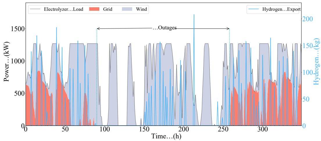
Figure 7: Case III (wind+battery+hydrogen+fuel cell+grid) electrolyzer load balance from different components, during both normal and grid outage periods. The right y-axis shows the hydrogen export volume.
