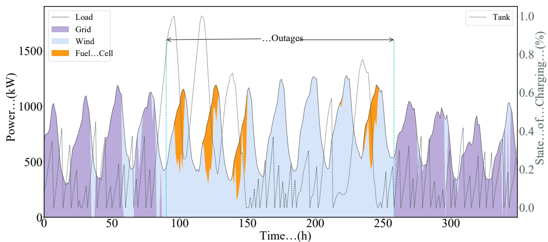
Figure 6: Case III (wind+battery+hydrogen+fuel cell+grid) load balance from different components, during both normal and grid outage periods. The right y-axis illustrates the state of charge of the hydrogen tank.
