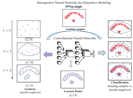
Figure 4. Schematic illustration of the pipeline of INNg-single.
