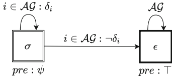
Fig. 2. Edge-conditioned update model for an ontic action
