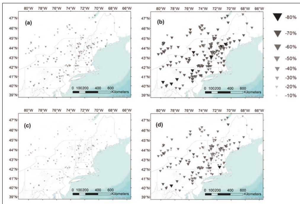
Figure 4. Percentage change in snowmaking days (minimum temperature < -5^{\circ}\text{C} ), 2006–2009, for 1 November–25 December under (a) RCP4.5 and (b) RCP8.5, and for November 1 through February 28 under (c) RCP4.5 and (d) RCP8.5. Percentage change estimated from Sen slope, 2006–2009, relative to historical baseline (1980–2005).
