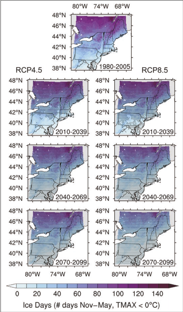
Figure 3. Cold-season (1 November–31 May) ice days (maximum temperature < 0\text{ }^{\circ}\text{C} ) climatology for historical (top), early (2010–2039), mid- (2040–2069), and late (2070–2099) century. Columns and stippling are as indicated in Figure 2.
