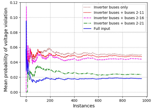
Fig. 12. Mean sampled probabilities of voltage violations for the probabilistic formulation with \alpha = 0.5 during training over 12–4 pm. The dimension of the DNN input increases as the number of nodes monitored in real time increases.
