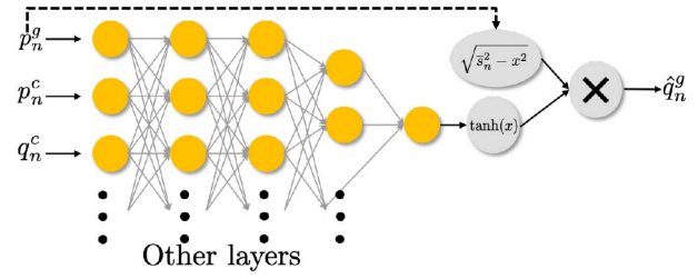
Fig. 2. The inverter control policy \mathbf{q} = \pi(\phi; \mathbf{w}) \in \mathcal{Q}_\theta has been implemented using a DNN. Vertically stacked nodes represent the nonlinear activation functions of a single layer. Edges across nodes correspond to weights applied linearly on node output to compute the inputs to the next layer. The vector of grid conditions \theta (or its proxy \phi ) is fed as the input to the DNN. Vector \mathbf{w} collects all weights of the DNN. The DNN output provides the inverter setpoints \mathbf{q} . The activation function of the output layer of the DNN has been modified to ensure \pi(\phi; \mathbf{w}) \in \mathcal{Q}_\theta for all \phi . The output neuron feeds into the \tanh(\cdot) activation function and then scaled by \sqrt{\bar{s}_n^2 - (p_n^g)^2} . The scaling operation involves a skip connection from p_n^g , which is one of the inputs to the DNN.
