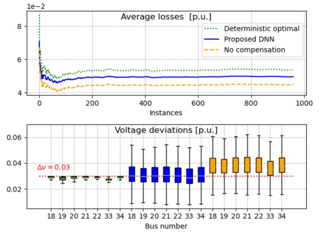
Fig. 6. Top : Time-averaged losses during the 12–4 pm training interval attained by the deterministic optimal control strategy of (2); the proposed DNN-based inverter control; and no reactive power compensation by inverters. Bottom : Box plots showing the first and third quantiles of the voltage deviations experienced across buses under the three control strategies. Due to high solar generation, the feeder experiences lower ohmic losses at the expense of severe over-voltages if there is no reactive power control by inverters. The deterministic optimal inverter control strategy regulates voltages by absorbing reactive power, which increases line currents and consequently losses. The proposed strategy achieves lower average losses over deterministic optimal inverter control as voltages are not constrained within \pm 3\% at all times.
