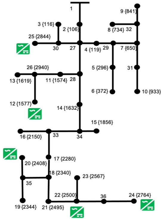
Fig. 5. The IEEE 37-bus feeder used for the numerical tests. Node numbering follows the format node number {panel ID}. The inverters at nodes {12, 20, 22, 24, 25} provide reactive power control, whereas the rest operate at unit power factor.
