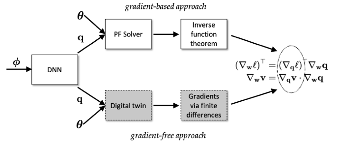
Fig. 4. Steps for calculating \nabla_{\mathbf{w}} \ell and \nabla_{\mathbf{w}} \mathbf{v} for the gradient-based (top) and gradient-free (bottom) approaches. The gradient-based approach requires a solution to the power flow equations in conjunction with the inverse function theorem (Section III); the gradient-free obtains the desired quantities by probing the digital twin and applying zero-order approximations.
