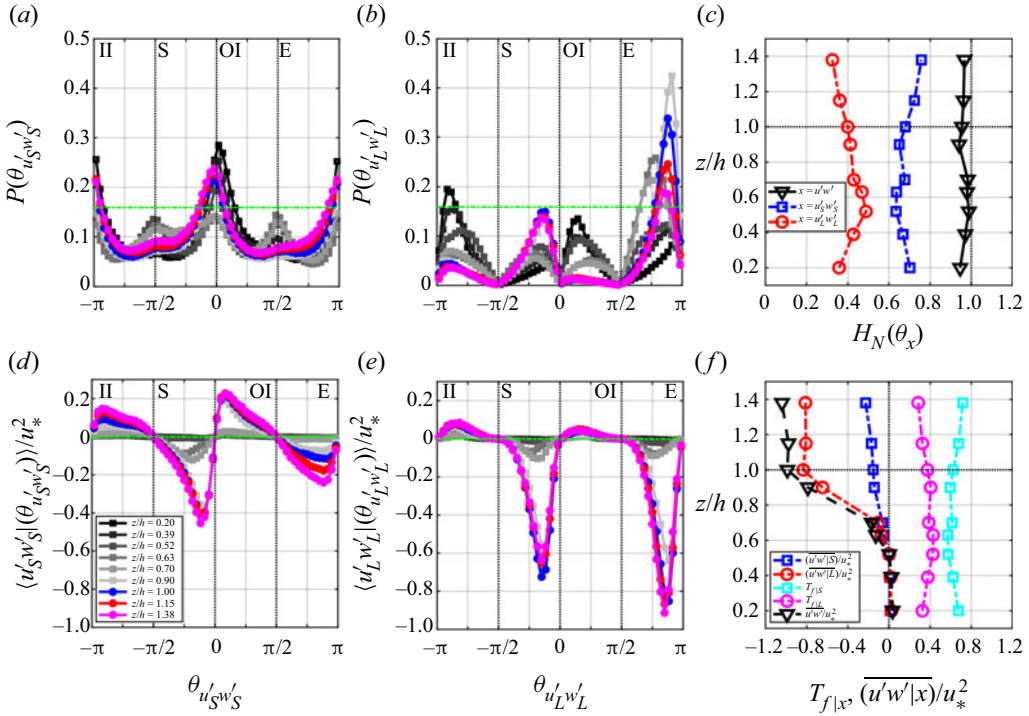
Figure 7. (a,b) P.d.f.s of quadrant angles for events whose duration remains in the range (a) t_p/\Gamma_w < 1 (short, u'_S w'_S ) and (b) t_p/\Gamma_w \geq 1 (long, u'_L w'_L ). (c) Normalized Shannon entropies of the quadrant angles for the two event classes. (d,e) Quadrant distributions of the momentum flux for the two event classes. (f) The contributions to the time fractions and momentum fluxes from the short- (S) and long-lived (L) events.
