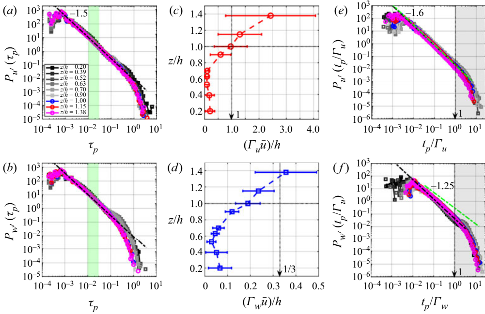
Figure 4. (a,b) Persistence p.d.f.s for the events in (a) u' and (b) w' , corresponding to the heights within and above the canopy. The normalized persistence time scales (t_p u_*)/h are denoted as \tau_p and their p.d.f.s are constructed over the ensemble of 93 half-hour blocks from near-neutral conditions. A power law of exponent -1.5 is fitted to the persistence p.d.f.s of u' events and shown as dash-dotted black lines. The green shaded regions in (a,b) denote the range of \bar{\tau}_p , over which it varies across the nine heights. (c,d) Vertical profiles of normalized integral time scales (\Gamma_x, \text{ where } x = u \text{ or } w) for u' and w' signals, respectively. (e,f) Persistence p.d.f.s of u' and w' , but where the time scales ( t_p ) are normalized by \Gamma_x . The grey shaded regions in (e,f) correspond to time scales t_p/\Gamma_x \geq 1 . The power laws with exponents -1.6 and -1.25 (dash-dotted green lines) are fits redrawn from the SLTEST data (Chowdhuri et al. 2020a).
