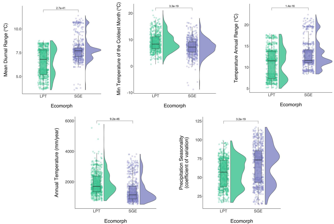
Extended Data Fig. 10 | Comparison of CHELSA climate variables that differ significantly between V. jucundum (LPT) and V. lautum (SGE) across the geographic range of Oreinotinus . Compared across the entire geographic range of Oreinotinus , LPT and SGE species differ significantly from one another in ways that align with our more detailed studies V. jucundum and V. lautum . Specifically, SGE species differ significantly from LPT species in their tendency to experience lower precipitation throughout the year, higher precipitation seasonality and higher seasonal and diurnal temperature ranges; SGE species may also tend to experience lower minimum temperatures in the coldest month. Viburnum jucundum and V. lautum were compared in detail on the Central Plateau of Chiapas, Mexico (see Fig. 4). In making comparisons across the range of Oreinotinus , we used data for the entire geographic ranges of these focal species (that is, extending beyond the central Plateau of Chiapas; see Extended Data Fig. 3. Hypothesis testing method, box plot elements and density ridges formulation as in Extended Data Fig. 8. N=1367 (713 LPT and 654 IGE specimens).
