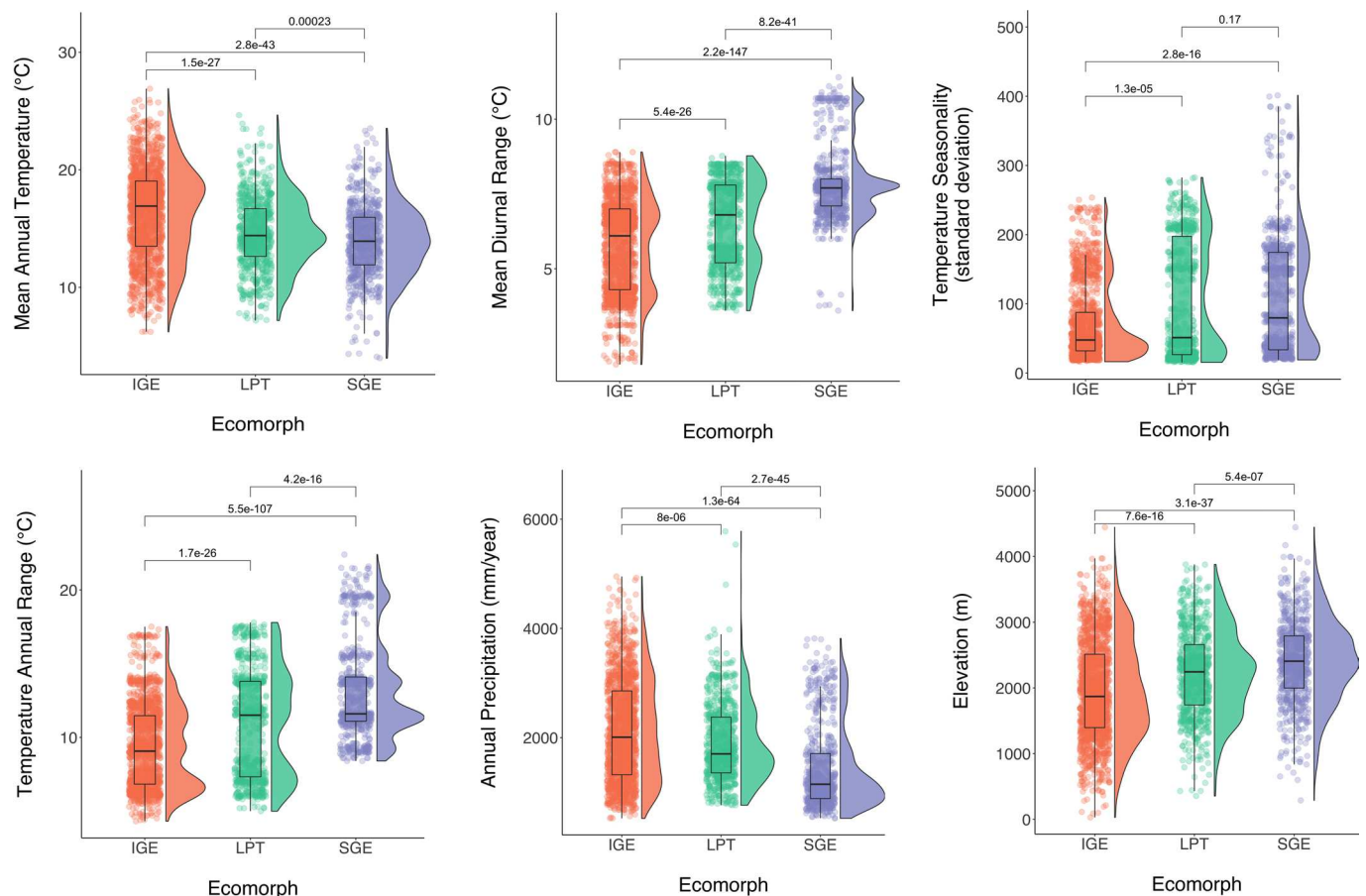
Extended Data Fig. 9 | Comparison of CHELSA climate variables that differ significantly in comparing V. hartwegii (IGE) to V. jucundum (LPT) and V. lautum (SGE) across the geographic range of Oreiotinus . Compared across the entire range of Oreiotinus , IGE species differ significantly from LPT and SGE species in ways that align with our findings for the niches of the V. hartwegii in comparison with V. jucundum and V. lautum (see Methods). Specifically, we find that IGE species grow at lower elevations with higher temperatures and higher precipitation throughout the year, and lower temperature ranges and seasonality. Viburnum hartwegii was compared in detail with V. jucundum and V. lautum on the Central Plateau of Chiapas, Mexico (see Fig. 4). In making comparisons across the range of Oreiotinus we used data for the entire geographic ranges of our three focal species (that is, extending beyond the central Plateau of Chiapas; see Extended Data Fig. 3). Hypothesis testing method, box plot elements and density ridges formulation as in Extended Data Fig. 8. N = 2783 (1416 IGE, 713 LPT, 654 SGE specimens).
