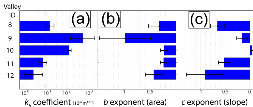
Figure 5. Bar plots of the k_b coefficient as well as b and c exponents in Eq. (2) for the reversed valley category (panels a , b , and c , respectively), fitted by multivariate regression. Error bars represent the 95 % confidence interval. The k_b values show large variability. The area exponents, b , are generally less negative than the d exponents fitted to Eq. (1) in Table 1 and Fig. 4. Except for valley 10, the slope exponents c have negative values. In valleys 8, 11, and 12, the c exponent is more negative than the area exponent, b , reflecting the key role of slope in reversed valley width prediction. Note the log scale of the x axis in panel ( a ).
