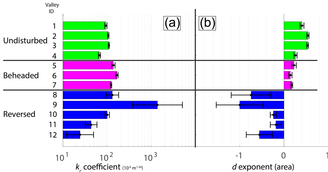
Figure 4. Bar plots of the k_c and d values ( a , b , respectively) for valley sections of the categories defined in Fig. 1c. The error bars represent the 95 % confidence interval. Unlike the k_c values, which lack a clear trend, the values of the d exponent ( b ) fall within a distinct range for each valley category. Note the log scale of the x axis in panel ( a ).
