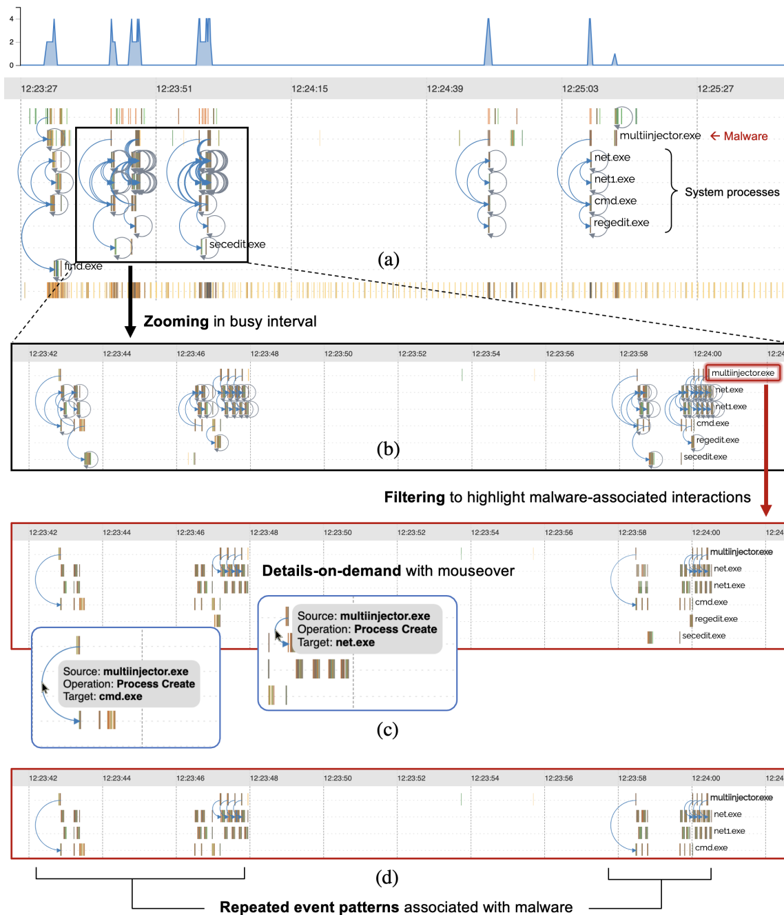
FIGURE 6. Trojan Multinjector under MalView analysis: the sequence of Process Create events generated by the malware and its interactions with other processes in the system.
