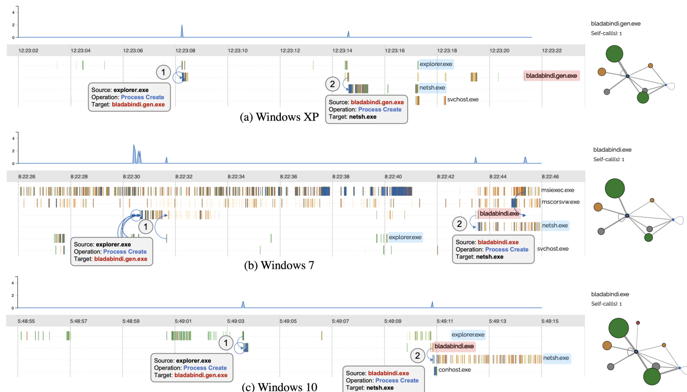
FIGURE 15. Patterns of malware behavior across platforms: Bladabindi malware executions Windows XP (a), Windows 7 (b) and Windows 10 (c), all under focus+context with busy interval length of 20 seconds. On the right end are the corresponding dependency graphs of the malware process. While different processes express different dependency graphs, as shown in Figure 5 and Figure 7, the dependency graph of Bladabindi malware is relatively consistent across different platforms.
