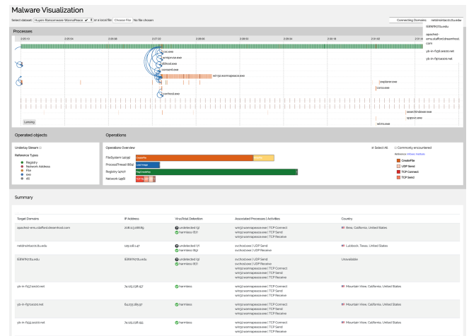
FIGURE 8. MalView analysis summary of ransomware WannaPeace on Windows 7.
