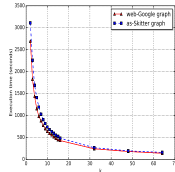
Figure 1: Performance of the distributed PageRank Algorithm of [21] on two graphs from Stanford Network Analysis Project (snap.stanford.edu): Google Web graph (875713 nodes) and Autonomous System by Skitter (1.69M nodes). The algorithm was implemented using MPI and run on a cluster of machines interconnected by a high speed network. The graph shows that the execution time is proportional (approximately) to 1/k^{0.8} .
