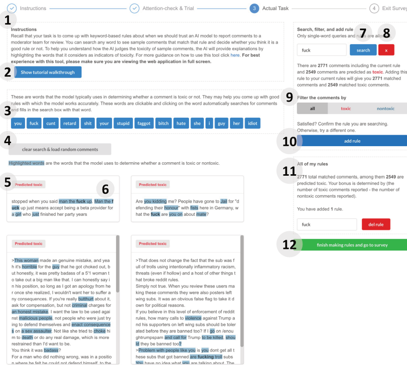
Figure 8: Interface for “Predicted label + local explanations + global explanations”. We use this interface to go through the design of all delegation support features.
