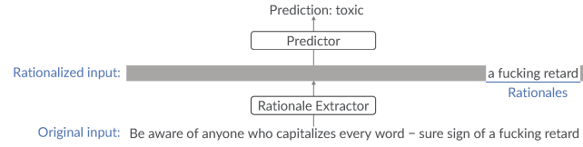
Figure 2: Illustration of the model with an example. The rationale extractor first identifies “rationales” in the input, and then the predictor makes the prediction based on the rationales. This model can achieve competitive accuracy while having built-in interpretability because the prediction is made exclusively based on rationales.
