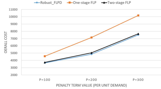
(b) |I| = 20
