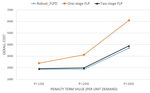
(a) |I| = 10
