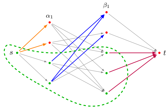
Fig. 9: We illustrate the three terms defined in (8). In this digraph, we let the cut (S, T) be such that the nodes depicted in green (resp. red) are nodes in S (resp. T ). The set S is circled by the dashed green line. Then, the term c(s, T_\alpha) is the sum of the capacities of the edges depicted in orange, the term c(S_\alpha, T_\beta) is the sum of the capacities of the edges depicted in blue, and the term c(S_\beta, t) is the sum of the capacities of the edges depicted in purple. The capacity of the cut (S, T) is easily seen to be sum of these three terms.
