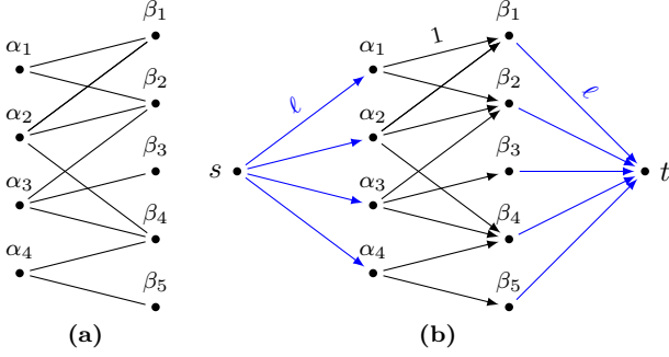
Fig. 5: Given a bipartite graph G(4,5) in (a), we plot the digraph \bar{G}(4,5) in (b). The edge set \bar{E} of \bar{G}(4,5) is partitioned into two subsets \bar{E}_0 and \bar{E}_1 depicted in blue and black, respectively. The capacity of each blue (resp. black) edge is \ell (resp. 1).
