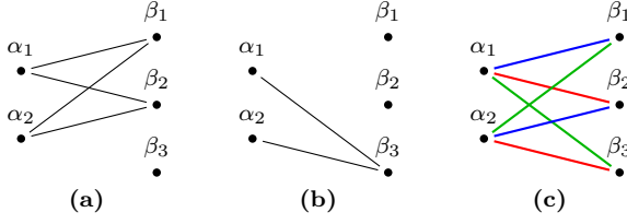
Fig. 7: In (a), we depict a graph G(2,3) which is the union of two disjoint left-perfect matchings P_1 = \{(\alpha_1, \beta_1), (\alpha_2, \beta_2)\} and P_2 = \{(\alpha_1, \beta_2), (\alpha_2, \beta_1)\} . In (b), we depict the complementary graph G^c(2,3) ; it does not contain a left-perfect matching. In (c), we plot the three disjoint left-perfect matchings in the complete bipartite graph K(2,3) = G(2,3) \cup G^c(2,3) .
