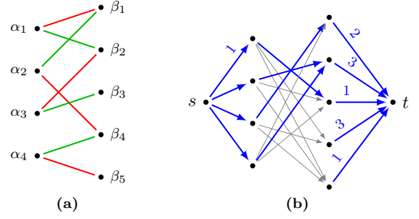
Fig. 8: The bipartite graph G(4,5) in (a) is a union of two disjoint left-perfect matchings, highlighted in red and green. The weighted digraph in (b) is G^c(4,5) for k = 3 . Correspondingly, by Def. 7, the capacity of an edge \beta_j t is given by 4 - \deg(\beta_j; G) , whereas the capacity of each remaining edge is 1. We then run the Ford-Fulkerson algorithm and highlight (in blue) a solution f to the max-flow problem (6). By Prop. 7, the capacity of any such solution is given by |f| = n = 4 .
