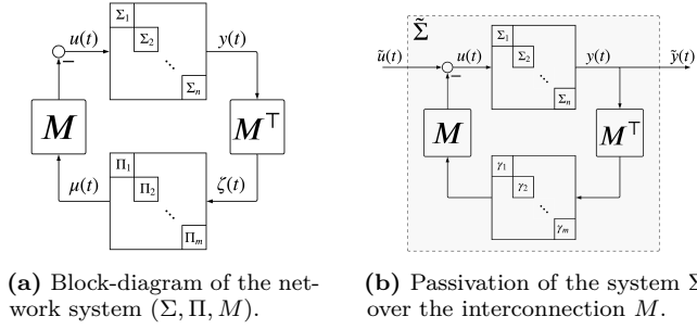
Fig. 1: A general network system and a network passivation approach.
