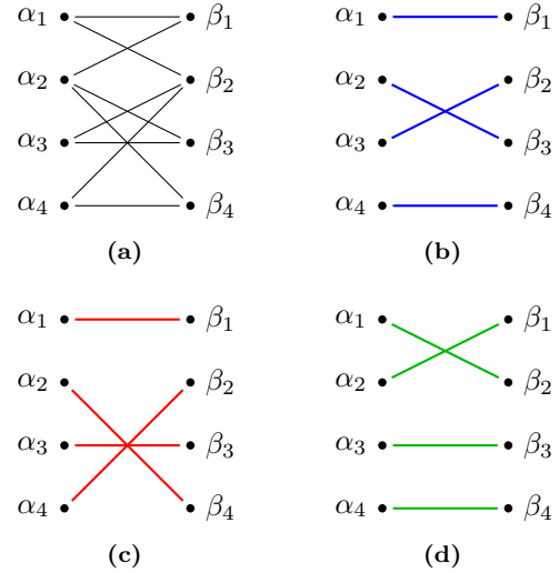
Fig. 4: The graph in (a) contains three distinct (but not pairwise disjoint) perfect matchings, depicted in (b)-(d). The intersection of these three perfect matchings is the empty set, i.e., there is no common edge to all these matchings. Hence, the graph in (a) is at least 1-resilient. Moreover, since \deg(\alpha_i) = \deg(\beta_i) = 2 for i = 1, 3, 4 , the graph in (a) is exactly 1-resilient. However, since the pairwise intersections of the matchings is not empty, it is not strongly 1-resilient.
