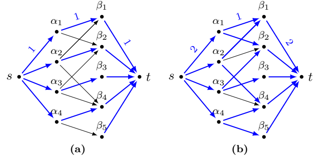
Fig. 6: We show saturated flows f_\ell on the graph \bar{G}(4, 5) as depicted in Fig. 5 for \ell = 1 in (a) and \ell = 2 in (b). The edges with nonzero values under f_\ell are highlighted in blue. In the case \ell = 2 , the two disjoint left-perfect matchings are \{(\alpha_1, \beta_1), (\alpha_2, \beta_4), (\alpha_3, \beta_2), (\alpha_4, \beta_5)\} and \{(\alpha_1, \beta_2), (\alpha_2, \beta_1), (\alpha_3, \beta_3), (\alpha_4, \beta_4)\} . Note, in particular, that the perfect matching of case \ell = 1 is not part of the disjoint matchings for \ell = 2 .
